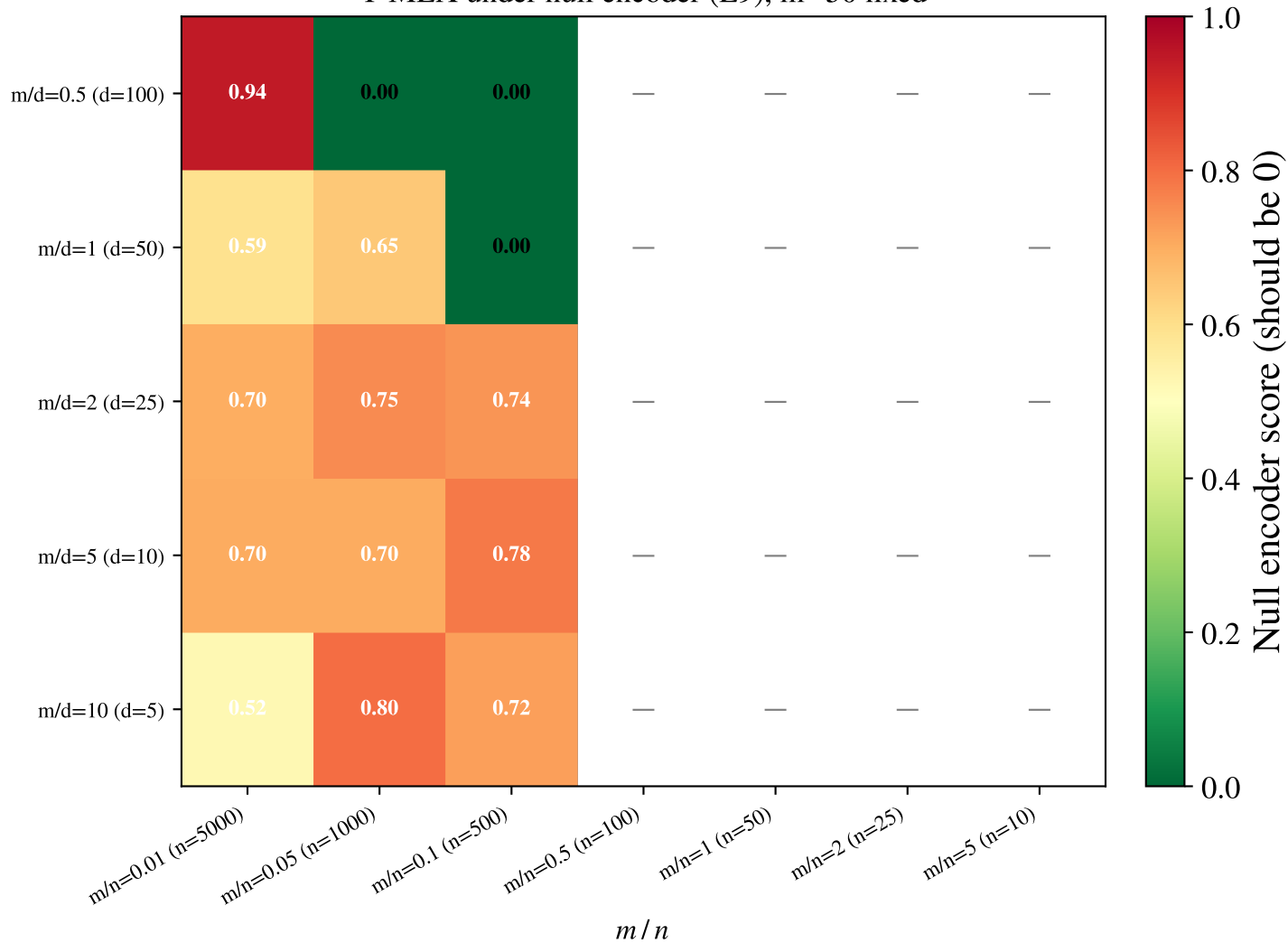
T-MEX under null encoder (E9), m=50 fixed
