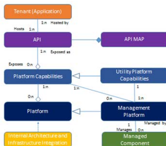
Figure 15 – Platform meta-model
