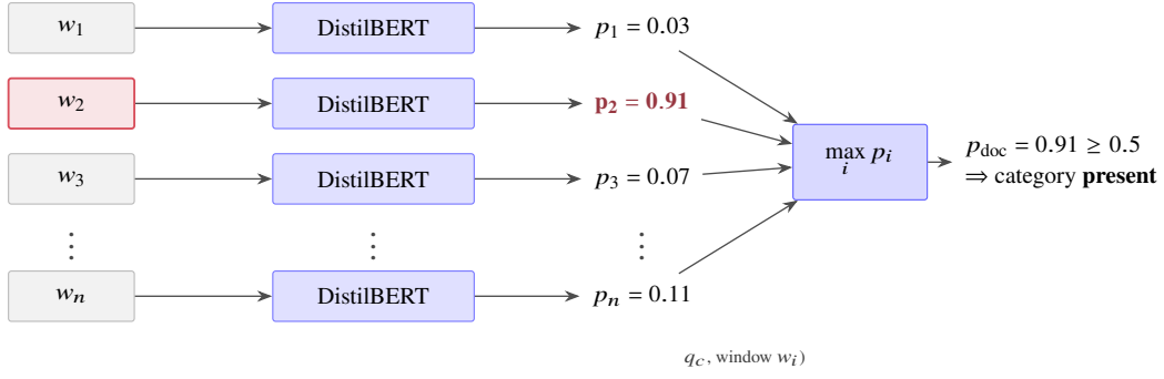
Figure 4.4: The multiple-instance learning rule: maximum over window scores.
