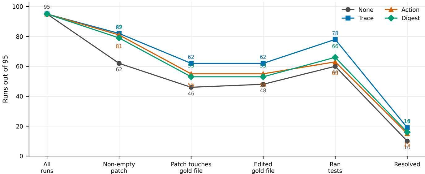
Action funnel across repair trajectories
