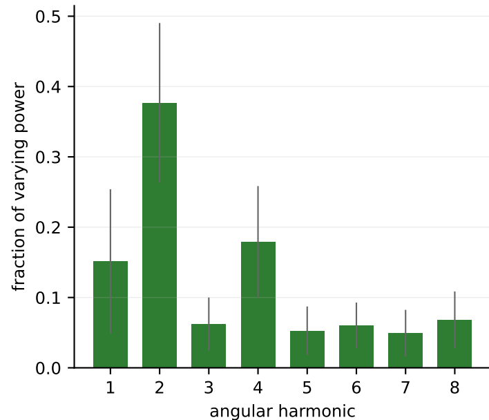
Orbit harmonic content (harmonic 0 holds 0.809 of total power)
