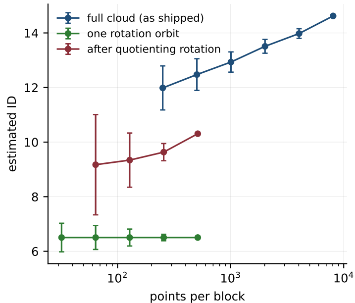
Block analysis: does the estimate move with N?
