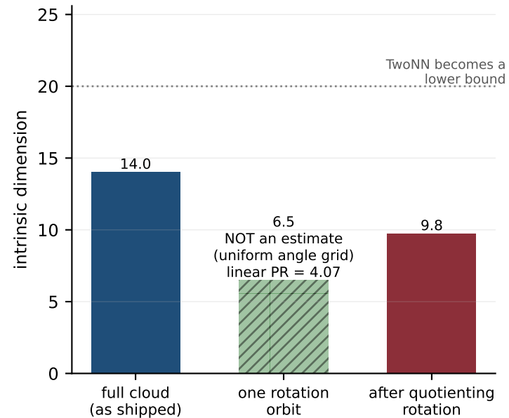
Dimensionality budget (twonn)
