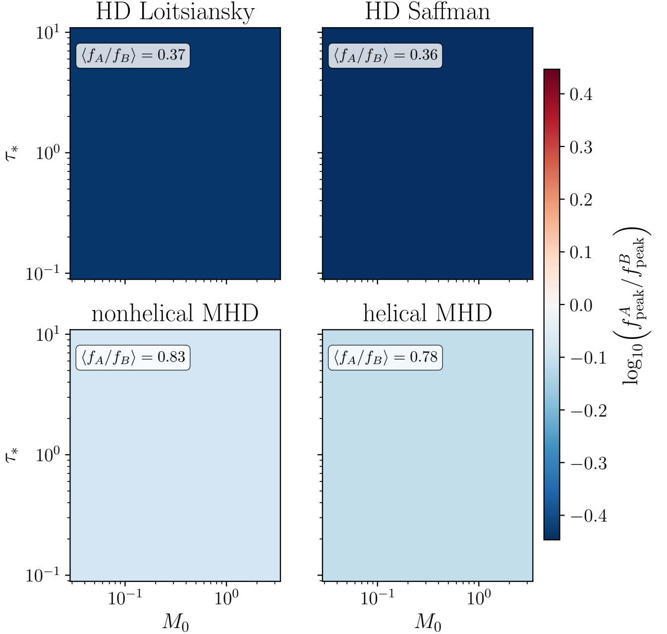
FIG. 5. Model A/B ratio of the peak GW frequency, \log_{10}(f_{\text{peak}}^A / f_{\text{peak}}^B) , on the (\tau_*, M_0) plane for the four BK2016 self-similar decay classes (HD Loitsiansky q = 2/7 , \beta = 4 ; HD Saffman q = 1/3 , \beta = 3 ; nonhelical MHD q = 1/2 , \beta = 1 ; helical MHD q = 2/3 , \beta = 0 ). Each panel is flat: the ratio is independent of (\tau_*, M_0) , fixed only by the kernel shapes, with the per-class value \langle f_A/f_B \rangle annotated. Model A (random-phase) peaks below Model B (coherent eddy) everywhere; the HD classes show the larger offset.
