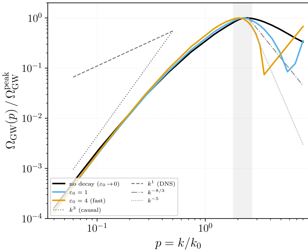
full-spatial self-similar spectra (wide p )
