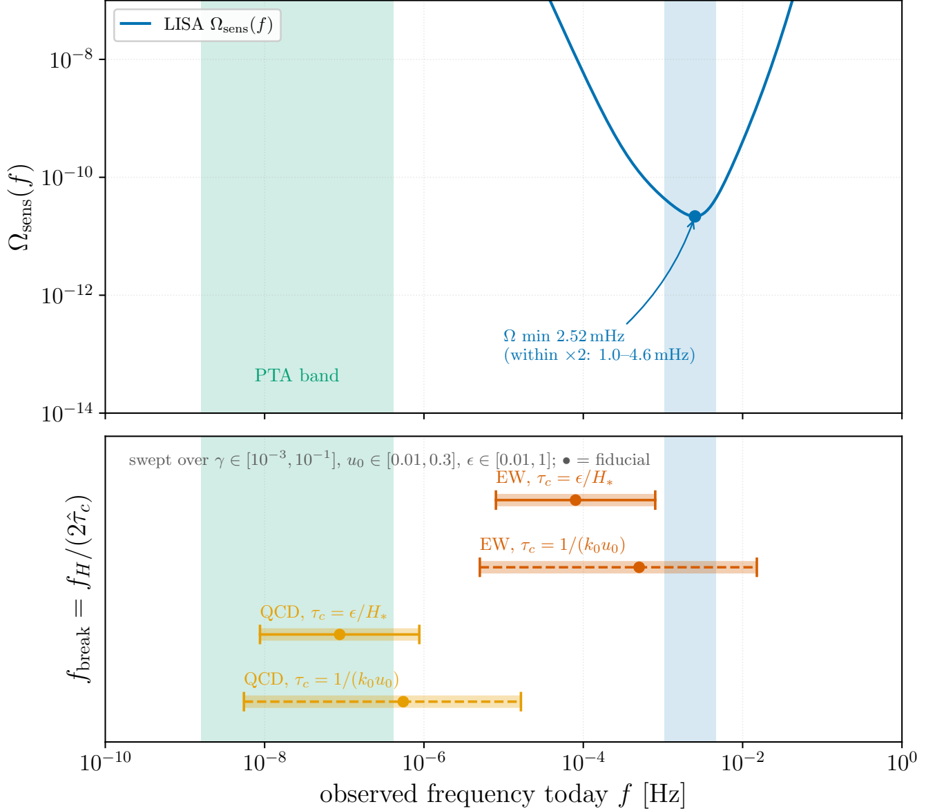
FIG. 15. Where the break falls relative to the observing bands. Top: the LISA energy-density sensitivity \Omega_{\text{sens}}(f) from the SciRD analytic noise model, with its minimum at 2.52 mHz and the factor-of-two window shaded, and the pulsar-timing band. Bottom: f_{\text{break}} swept over the parameter ranges of Table V for the two epochs and the two lifetime closures. The bands are two to three decades wide, which is the point: the break’s position relative to each instrument is robust where its value is not. Generated by Notebooks/k_break_frequency.py .
