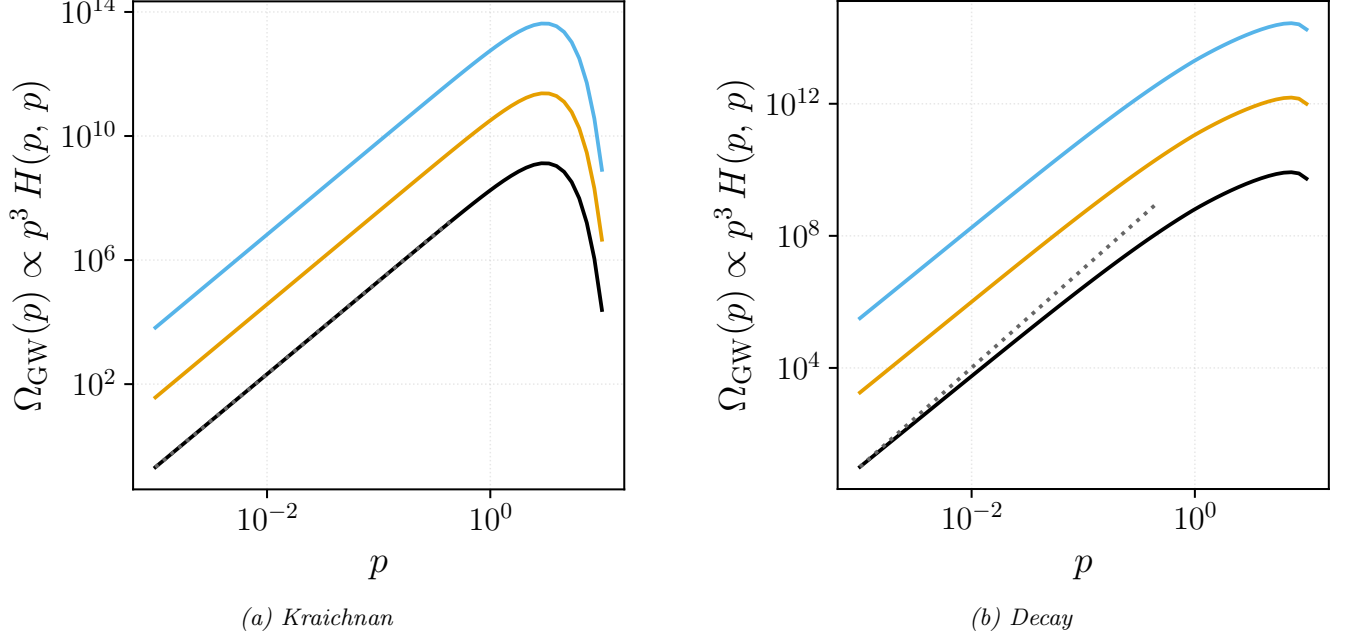
FIG. 10. White-noise real-space correlations R_{ij} \propto \delta^{(3)}(\mathbf{r}) . Three curves per panel correspond to R = 10^3, 10^4, 10^5 . Panel (a): Kraichnan decorrelation, matches the universal IR slope 3 . Panel (b): decay temporal model, IR slope 1.3 (flagged: temporal-convolution tails pull power down at small p ).
