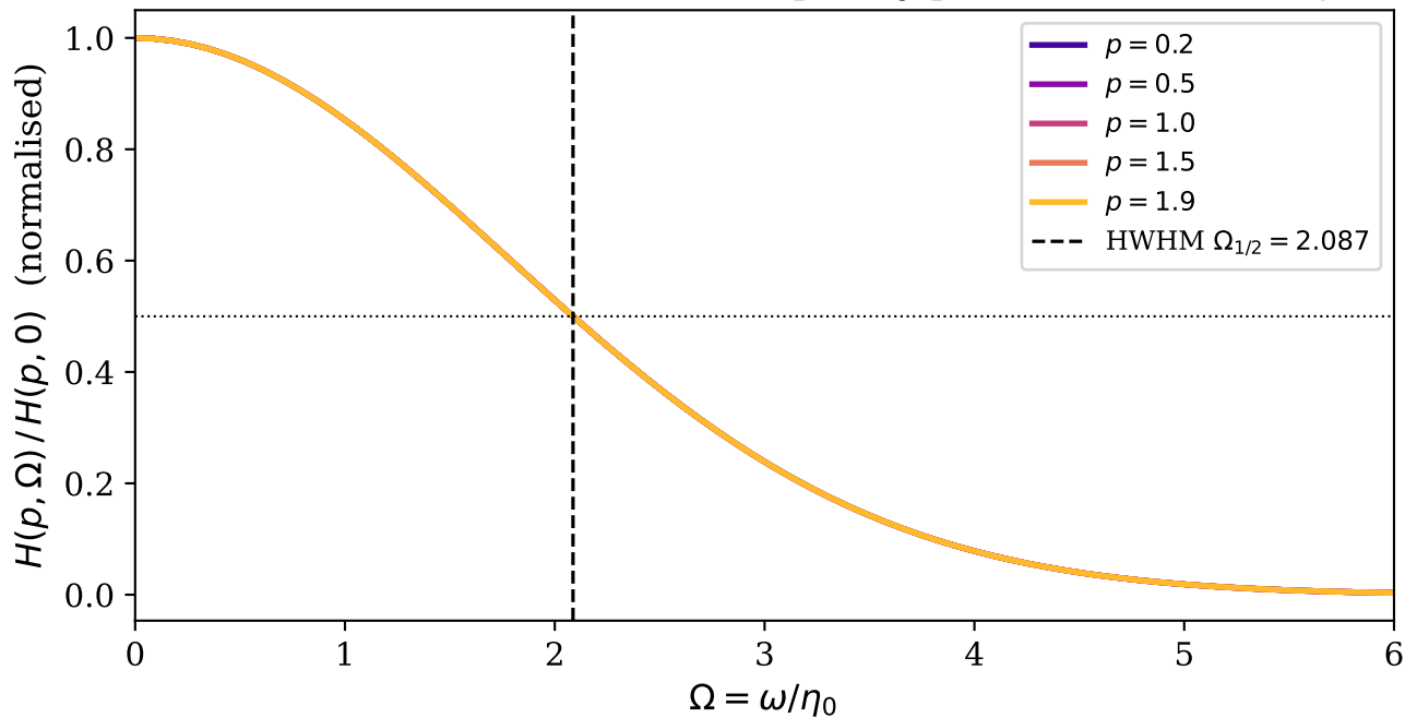
Delta-k Kraichnan: Gaussian frequency profile (same for all p )
