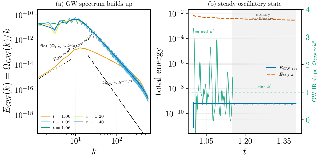
FIG. 12. Time-series reanalysis of the Roper Pol et al. [28] run ini2 (public Pencil Code spectra, Zenodo 10.5281/zenodo.3692072), the run of their Fig. 1. (a) The GW energy spectrum E_{\text{GW}} = \Omega_{\text{GW}}/k at successive times: at switch-on ( t \simeq 1.0 ) the infrared follows the causal E_{\text{GW}} \sim k^2 ( \Omega_{\text{GW}} \sim k^3 ) and within \Delta t \sim 0.02 saturates to the flat plateau ( \Omega_{\text{GW}} \sim k^1 ) of their Fig. 1. (b) Total energies versus time: the GW energy rises while the source acts, then fluctuates about a steady mean (grey band; the “steady oscillatory state”), while the magnetic energy keeps decaying; the right axis (green) shows the measured GW infrared slope crossing from the causal k^3 to the saturated k^1 . Generated by Notebooks/roperpol_timeseries.py , which auto-downloads the data.
