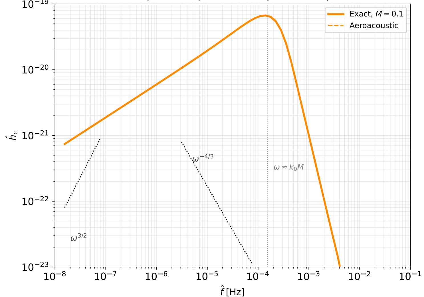
GW spectral shape: M = 0.1 — predicted slopes
