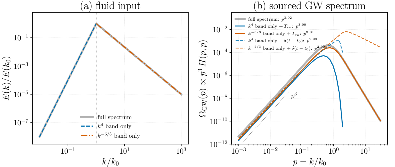
FIG. 14. Band-split test of the white-noise-floor hypothesis. (a) The three fluid inputs fed to the kernel: the full spectrum of Eq. (24) (grey), its Batchelor band E \propto k^4 alone (blue, dashed) and its Kolmogorov range E \propto k^{-5/3} alone (orange, dash-dotted), obtained by masking the shape factor S(k) = A(k)/A_{\text{Kol}}(k) on one side of k_0 (dotted vertical line). (b) The gravitational-wave spectra \Omega_{\text{GW}}(p) \propto p^3 H_{ijij}(p, p; M, R) they source on the sound-cone diagonal q = p , with the infrared log-log slopes fitted over 2 \times 10^{-3} \leq p \leq 2 \times 10^{-2} quoted in the legend; the dotted guide is p^3 . All are causal to better than 2% in the exponent, including the inertial-range-only run, whose input has no infrared power at all. The Batchelor-only spectrum ends at p = 2 , the kinematic limit of a convolution of two modes with k < k_0 . The two dashed curves repeat the single-band runs with the temporal factor removed entirely—evaluated at q = 0 rather than on the diagonal q = p , so that the Gaussian sweeping factor and its erfc in Eq. (22) are both unity and the source carries no decorrelation and no time dependence at all [the impulsive limit, Eq. (B105)]. The spatial integral is otherwise identical, so each solid/dashed pair isolates what the temporal model does and does not control. Parameters: M = 0.5 , R = (k_d/k_0)^{4/3} = 10^4 , R_{\text{IR}} = k_0/k_{\text{IR}} = 10^2 , Batchelor infrared slope s = 4 . Both panels are dimensionless and the vertical offset between them carries no physical meaning. Produced by Notebooks/band_split_gw.py .
