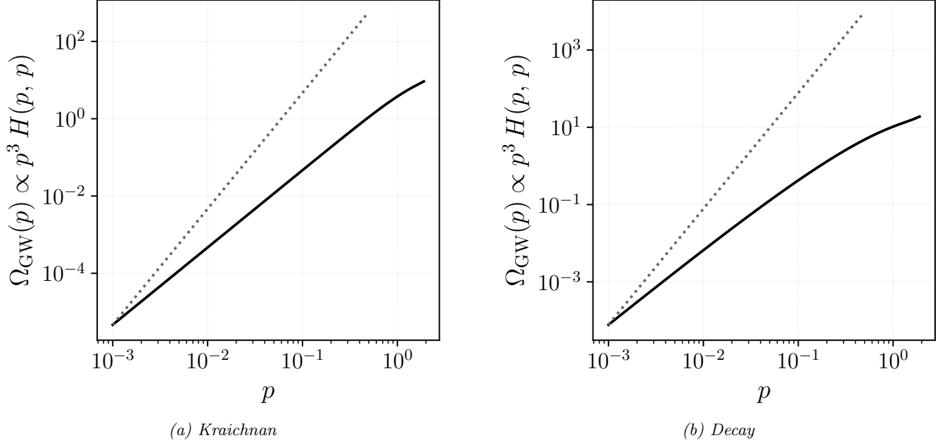
FIG. 19. Monochromatic spectrum E(k) = E_0 \delta(k - k_0) (no free parameters at the dimensionless level). Panel (a): Kraichnan decorrelation, closed form \Omega_{\text{GW}}(p) \propto p^3 K_0(p)/p \Theta(2-p) e^{-p^2/(2\pi)} with IR slope 2 (flagged: 1/p pole from the monochromatic source removes one power of p from the universal scaling). Panel (b): decay temporal factor, Eq. (C8), IR slope 2 — the same slope as panel (a), as it must be, since the temporal factor tends to the constant \pi \mathcal{C}(0) as p \rightarrow 0 and so cannot alter the infrared scaling.
