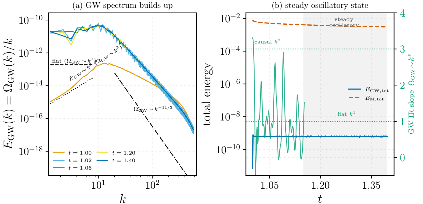
FIG. 11. Time-series reanalysis of the Roper Pol et al. [26] run ini2 (public Pencil Code spectra, Zenodo 10.5281/zenodo.3692072), the run of their Fig. 1. (a) The GW energy spectrum E_{\text{GW}} = \Omega_{\text{GW}}/k at successive times: at switch-on ( t \simeq 1.0 ) the infrared follows the causal E_{\text{GW}} \sim k^2 ( \Omega_{\text{GW}} \sim k^3 ) and within \Delta t \sim 0.02 saturates to the flat plateau ( \Omega_{\text{GW}} \sim k^1 ) of their Fig. 1. (b) Total energies versus time: the GW energy rises while the source acts, then fluctuates about a steady mean (grey band; the “steady oscillatory state”), while the magnetic energy keeps decaying; the right axis (green) shows the measured GW infrared slope crossing from the causal k^3 to the saturated k^1 . Generated by Notebooks/roperpol.timeseries.py , which auto-downloads the data.
