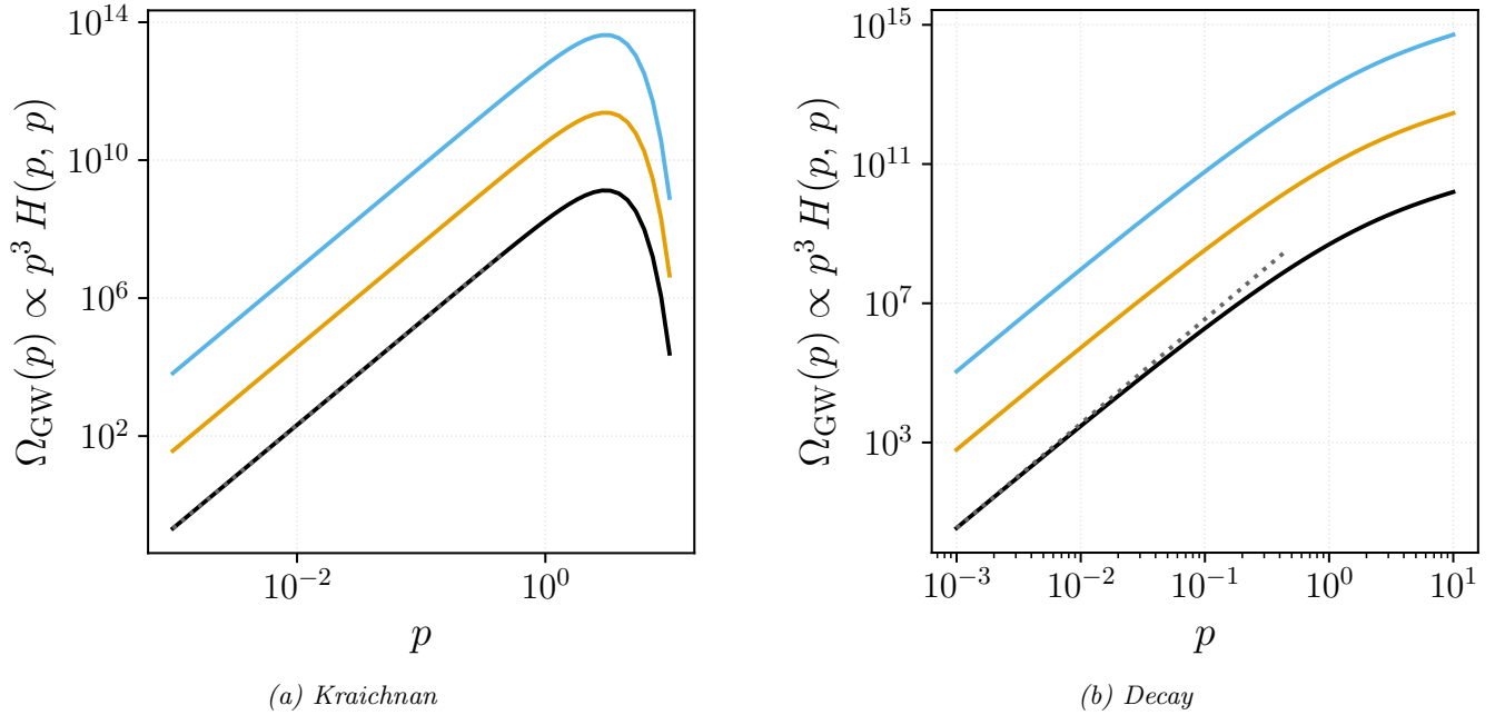
FIG. 20. White-noise real-space correlations R_{ij} \propto \delta^{(3)}(\mathbf{r}) . Three curves per panel correspond to R = 10^3, 10^4, 10^5 . Panel (a): Kraichnan decorrelation, matches the universal IR slope 3 . Panel (b): decay temporal model, IR slope 3 as well, for all three R — the decaying and Kraichnan models share the universal causal infrared, the temporal factor affecting only the amplitude and the ultraviolet tail.
