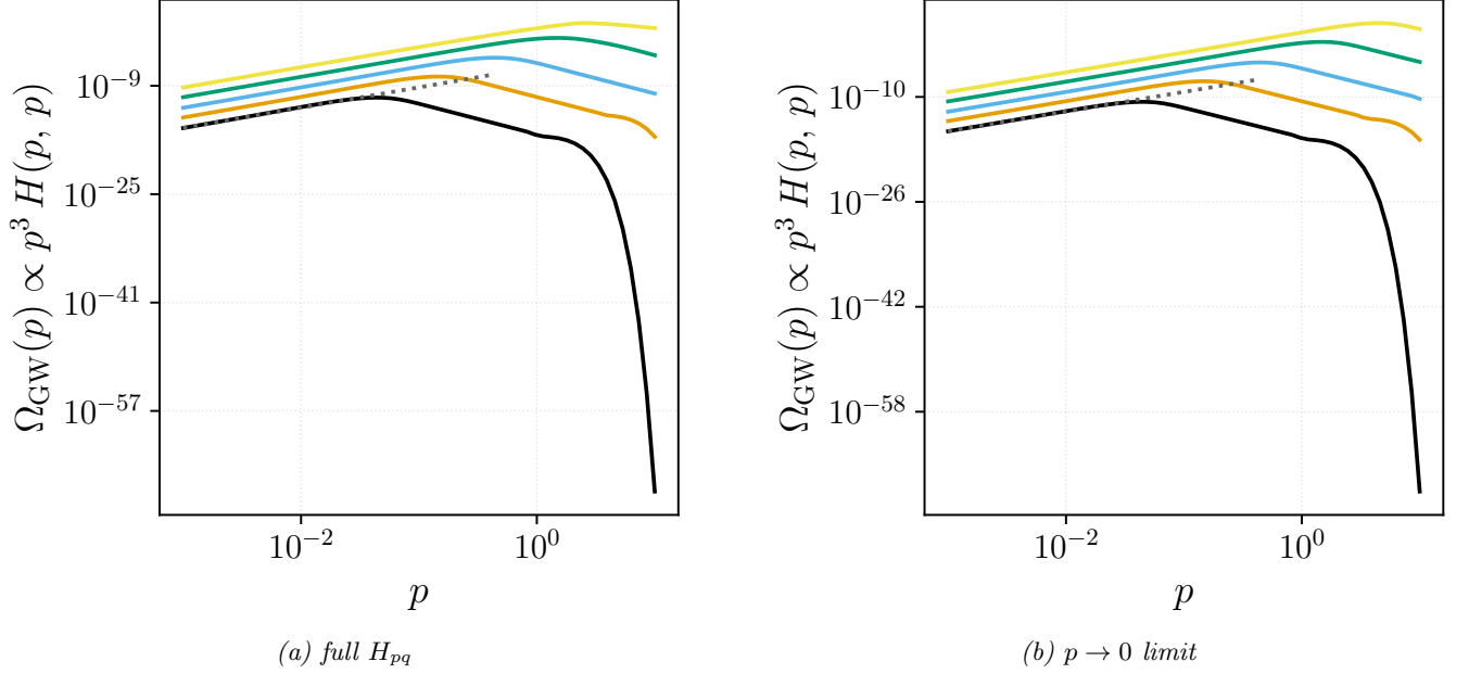
FIG. 18. Kraichnan decorrelation + Kolmogorov spectrum. Five curves per panel correspond to M = 0.03, 0.1, 0.3, 1.0, 3.0 at R = 10^4 . Panel (a) is the full numerical H_{pq} (Sec. III); panel (b) is the aeroacoustic p \rightarrow 0 limit (Kahnashvili et al. 2008). Both give the universal IR slope \Omega_{\text{GW}} \propto p^3 .
