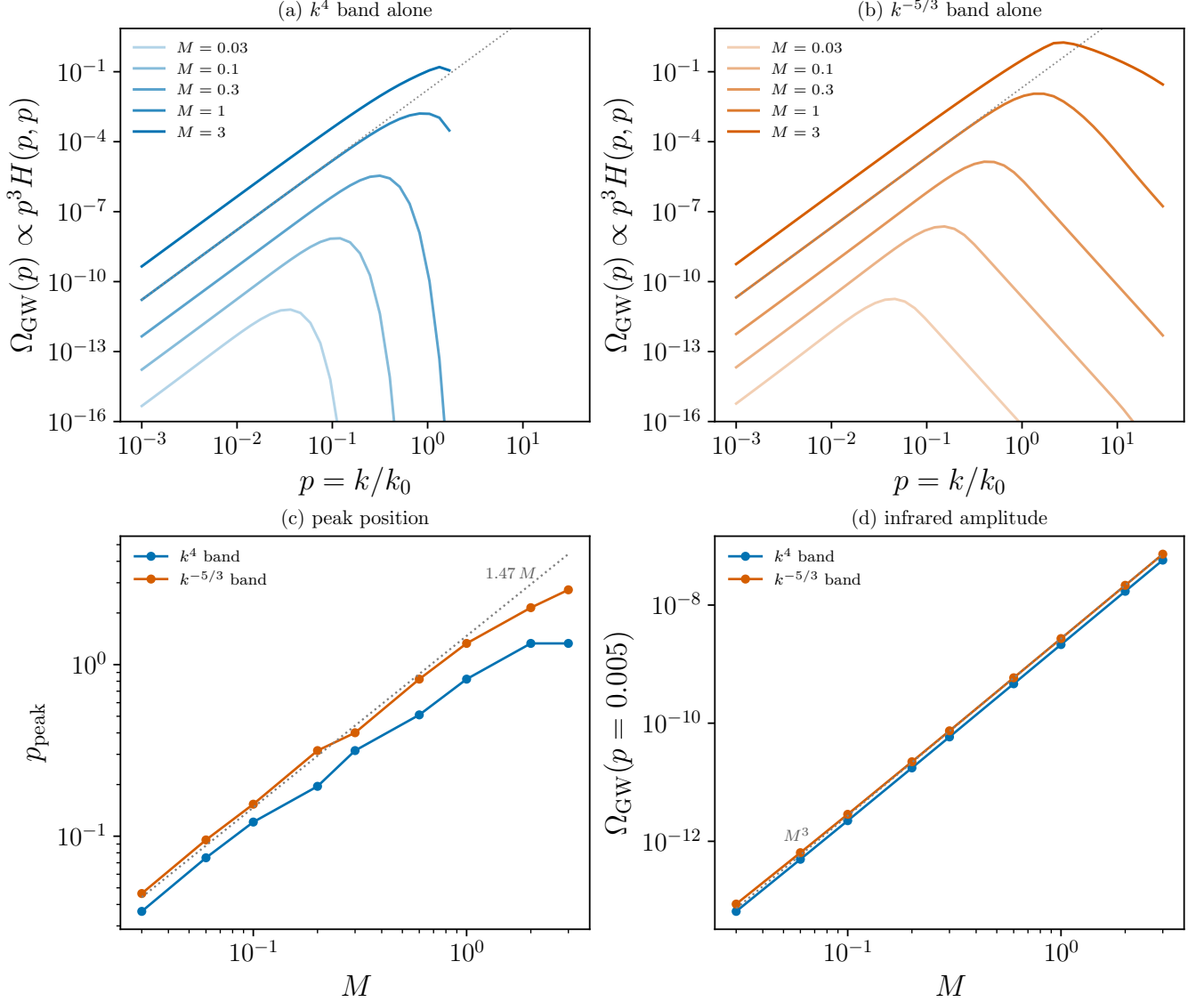
FIG. 15. Mach dependence of the band-split spectra, at R = 10^4 , R_{\text{IR}} = 10^2 , Kraichnan sweeping on the diagonal q = p . (a), (b) \Omega_{\text{GW}}(p) from the Batchelor k^4 band alone and from the Kolmogorov k^{-5/3} band alone, at M = 0.03, 0.1, 0.3, 1, 3 (increasing shade); dotted line p^3 . The infrared exponent is M -independent for both bands; the amplitude and the peak are not. (c) Peak position against M , with the 1.47 M sweeping law of Eq. (30) dotted. The inertial band reproduces it; the Batchelor band tracks a slightly lower 1.1 M and saturates above M \simeq 1 , where the sweeping scale meets the kinematic ceiling p \leq 2 that bounds a convolution of two modes with k < k_0 . (d) Infrared amplitude at p = 5 \times 10^{-3} against M , with the M^3 prefactor dotted; both bands follow it to 13% and 19% over two decades of M . Produced by Notebooks/band_split_mach.py .
