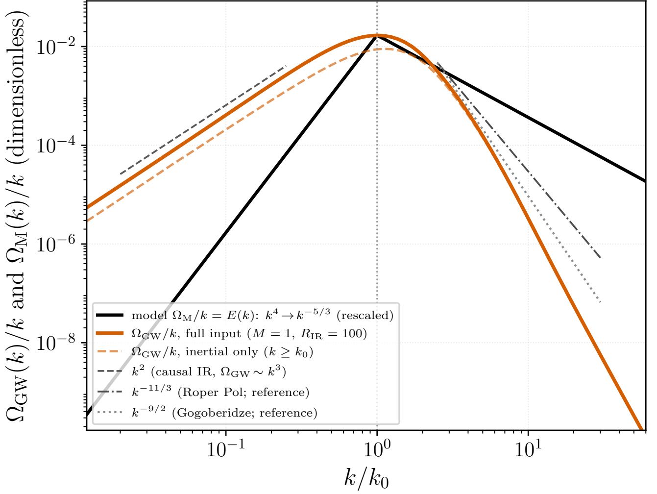
FIG. 2. Analytic spectra in the Roper Pol et al. [26] convention \Omega(k)/k = E(k) . Orange (solid): GW spectrum \Omega_{\text{GW}}(k)/k = p^2 H_{ijij}(p, p; M, R) [Eq. (23)] computed from a full fluid input spectrum—an infrared band E \propto k^4 ( k < k_0 ) joined to the Kolmogorov range E \propto k^{-5/3} ( k \geq k_0 ), Eq. (24)—fed into the Appendix-A kernel Eq. (19) through the shape factor S(k) = A/A_{\text{Kol}} ( M = 1 , R = 10^4 , infrared range R_{\text{IR}} = k_0/k_{\text{IR}} = 100 ). Orange (dashed): the same kernel restricted to the inertial range only ( R_{\text{IR}} = 1 , i.e. core Eq. (22))—the infrared band raises the amplitude near the peak but leaves the ultraviolet unchanged. Black: the full fluid input spectrum, rescaled to share the GW peak (the GW–fluid vertical offset is unphysical; only shapes compare). Grey dashed: the causal infrared guide k^2 ( \Omega_{\text{GW}} \sim k^3 ). Dash-dot/dotted: the k^{-11/3} (Roper Pol, run ini2) and k^{-9/2} (Gogoberidze) slopes reported in the literature, as references only—no simulation data points are plotted. At M = 1 the GW spectrum steepens past the peak to \simeq k^{-5.0} , steeper than both references, independently of the infrared treatment. Generated by Notebooks/roperpol_convention_spectra.py .
