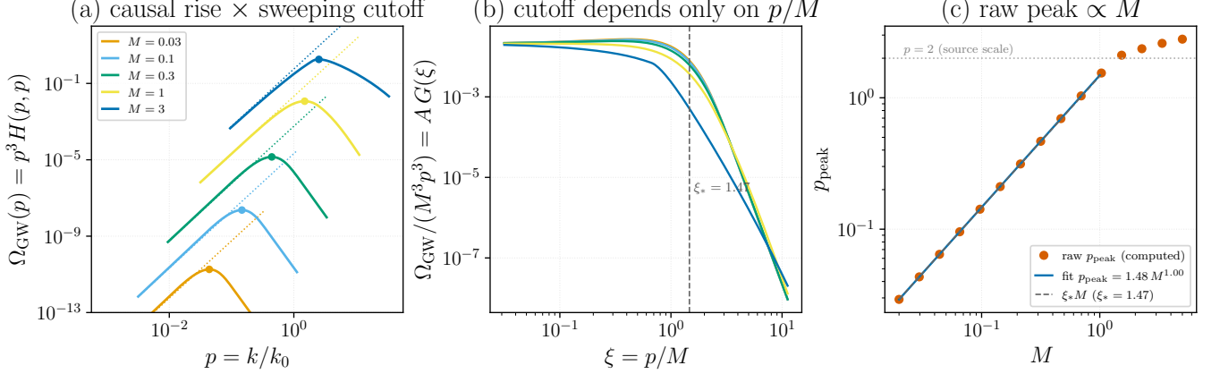
FIG. 3. Why the stationary GW spectrum peaks at p \simeq 1.47 M rather than at the source scale p \sim 2 , computed from \Omega_{\text{GW}}(p) = p^3 H_{ijij}(p, p; M, R) [Eq. (22), R = 10^4 ]. (a) Each spectrum (solid) follows its causal infrared asymptote A M^3 p^3 (dotted) and rolls over at the peak (dot) where the sweeping cutoff switches on. (b) Collapse: \Omega_{\text{GW}}/(M^3 p^3) = H_{ijij}(p, p; M)/M^3 versus \xi = p/M falls on the single compensated kernel \tilde{H}_{ijij}(\xi) for every M , proving the cutoff depends only on p/M [Eq. (27)]; the universal peak position is \xi_* = 1.47 . (c) Peak location read directly from each computed spectrum (points) versus M : a power law p_{\text{peak}} = 1.48 M^{1.00} (line) [Eq. (30)], coincident with \xi_* M (dashed), that bends below it toward the p = 2 source scale (dotted) only as M \rightarrow 1 (the luminal limit; M > 1 is superluminal). Generated by Notebooks/stationary_peak_analysis.py .
