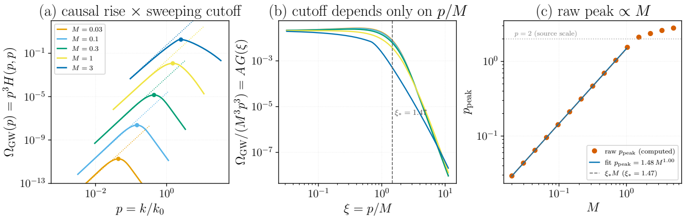
FIG. 3. Why the stationary GW spectrum peaks at p \simeq 1.47 M rather than at the source scale p \sim 2 , computed from \Omega_{\text{GW}}(p) = p^3 H_{ijij}(p, p; M, R) [Eq. (21), R = 10^4 ]. (a) Each spectrum (solid) follows its causal infrared asymptote A M^3 p^3 (dotted) and rolls over at the peak (dot) where the sweeping cutoff switches on. (b) Collapse: \Omega_{\text{GW}}/(M^3 p^3) versus \xi = p/M falls on a single curve AG(\xi) for every M , proving the cutoff depends only on p/M [Eq. (25)]; the universal peak position is \xi_* = 1.47 . (c) Peak location read directly from each computed spectrum (points) versus M : a power law p_{\text{peak}} = 1.48 M^{1.00} (line) [Eq. (28)], coincident with \xi_* M (dashed), that bends below it toward the p = 2 source scale (dotted) only at transonic M . Generated by Notebooks/stationary_peak_analysis.py .
