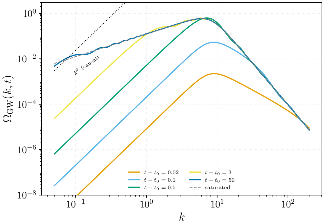
time-dependent GW spectrum: causal knee sweeps to low k
