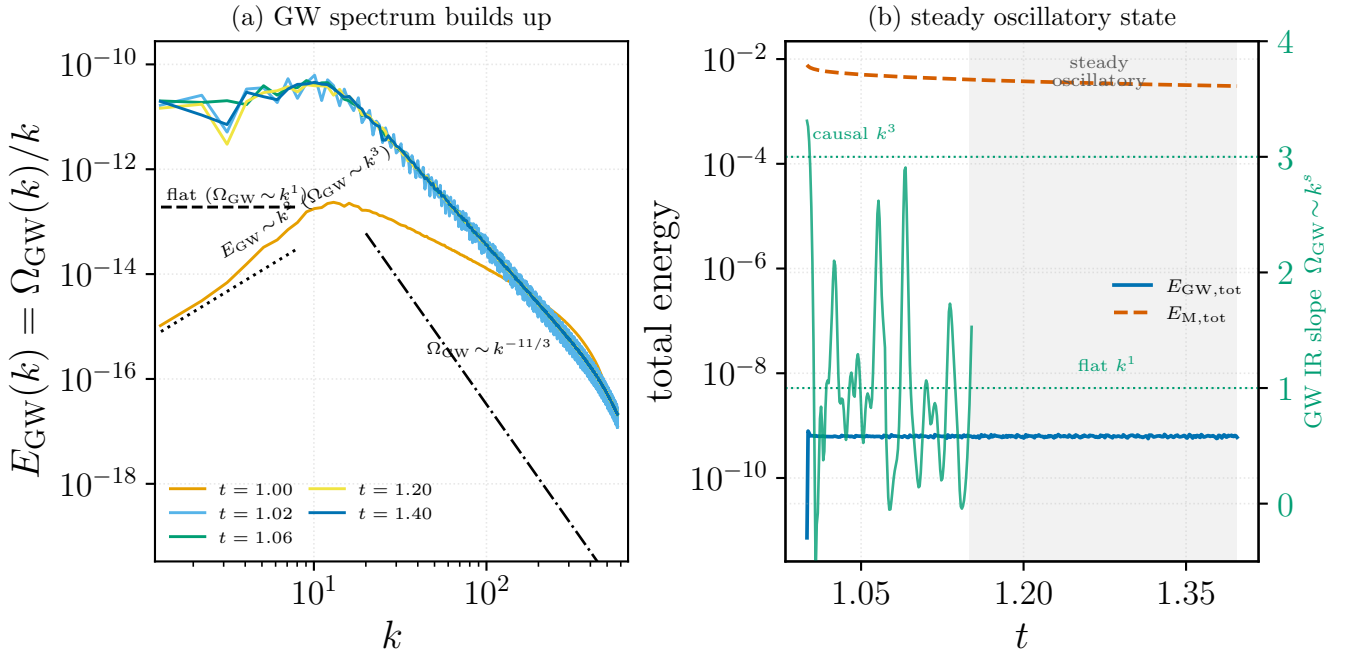
FIG. 11. Time-series reanalysis of the Roper Pol et al. [31] run ini2 (public Pencil Code spectra, Zenodo 10.5281/zenodo.3692072), the run of their Fig. 1. (a) The GW energy spectrum E_{\text{GW}} = \Omega_{\text{GW}}/k at successive times: at switch-on ( t \simeq 1.0 ) the infrared follows the causal E_{\text{GW}} \sim k^2 ( \Omega_{\text{GW}} \sim k^3 ) and within \Delta t \sim 0.02 saturates to the flat plateau ( \Omega_{\text{GW}} \sim k^1 ) of their Fig. 1. (b) Total energies versus time: the GW energy rises while the source acts, then fluctuates about a steady mean (grey band; the “steady oscillatory state”), while the magnetic energy keeps decaying; the right axis (green) shows the measured GW infrared slope crossing from the causal k^3 to the saturated k^1 . Generated by Notebooks/roperpol_timeseries.py , which auto-downloads the data.
