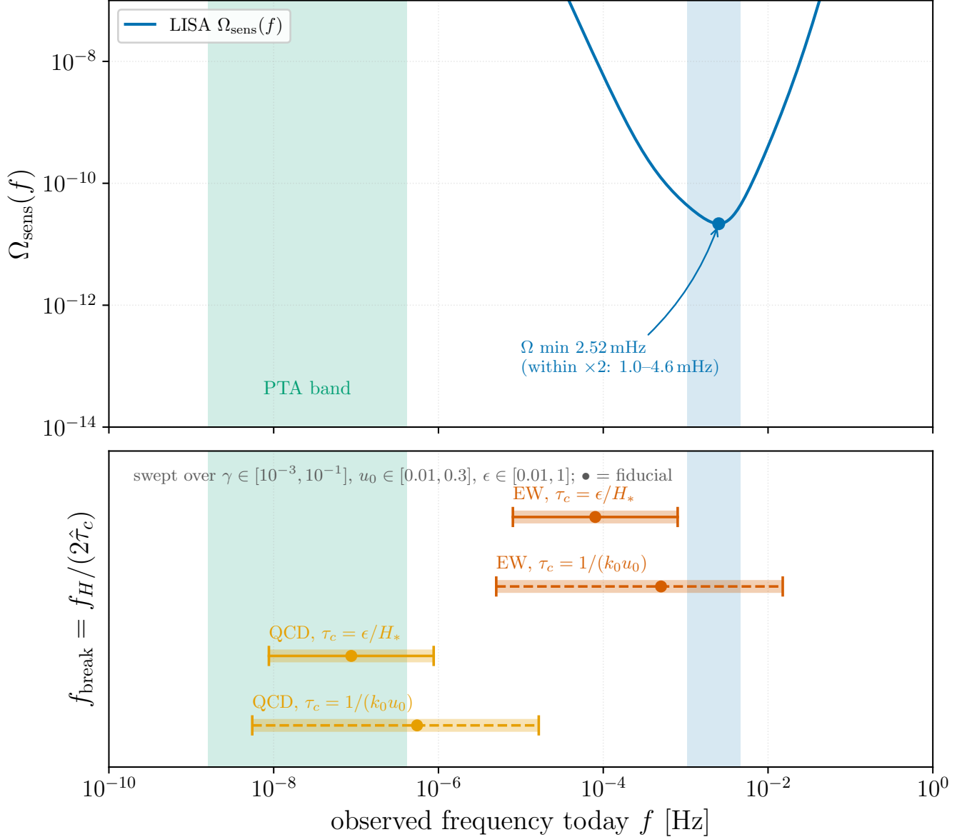
FIG. 16. Where the break falls relative to the observing bands. Top : the LISA energy-density sensitivity \Omega_{\text{sens}}(f) from the SciRD analytic noise model, with its minimum at 2.52 \text{ mHz} and the factor-of-two window shaded, and the pulsar-timing band. Bottom : f_{\text{break}} swept over the parameter ranges of Table VI for the two epochs and the two lifetime closures. The bands are two to three decades wide, which is the point: the break’s position relative to each instrument is robust where its value is not. Generated by Notebooks/k_break_frequency.py .
