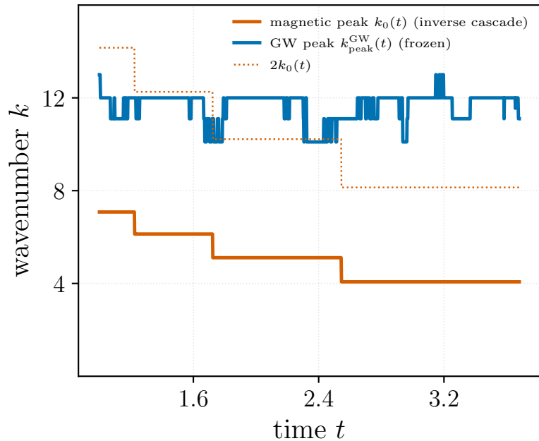
(b) k_0 cascades down, GW peak stays
