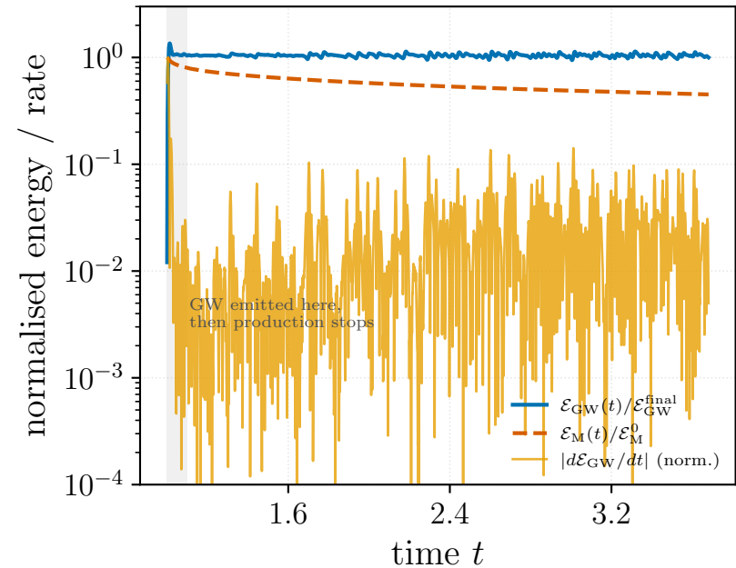
(a) GW production is impulsive
