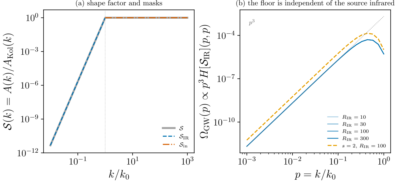
FIG. 21. The two ingredients of the band-split chain. (a) The shape factor \mathcal{S} of Eq. (B116) and its masks \mathcal{S}_{\text{IR}}, \mathcal{S}_{\text{in}} of Eq. (B117). The masks have disjoint support and sum to \mathcal{S} , so each traces it exactly on its own side of k_0 (dotted vertical); this is what makes the decomposition Eq. (B120) exact rather than approximate. (b) Eq. (B121) made visible: the infrared band alone, \Omega_{\text{GW}} \propto p^3 H[\mathcal{S}_{\text{IR}}](p, p) , at four infrared bandwidths R_{\text{IR}} = 10, 30, 100, 300 and at two infrared slopes s = 4 (Batchelor) and s = 2 (Saffman), with M = 0.5, R = 10^4 . The four bandwidth curves are drawn separately but are not distinguishable: they agree to 0.31% at p = 5 \times 10^{-3} despite spanning 1.5 decades of R_{\text{IR}} , because the floor P_T(0) = \int d^3 q P_M(q)^2 is fixed by the modes at the top of the band and is blind to how far the band extends. Changing the infrared slope itself moves the amplitude by only 2.71 and leaves the exponent at 3.005 against 3.001, although the two inputs differ by four decades at the bottom of the band. Dotted guide: p^3 . Produced by Notebooks/band_split_masks.py .
