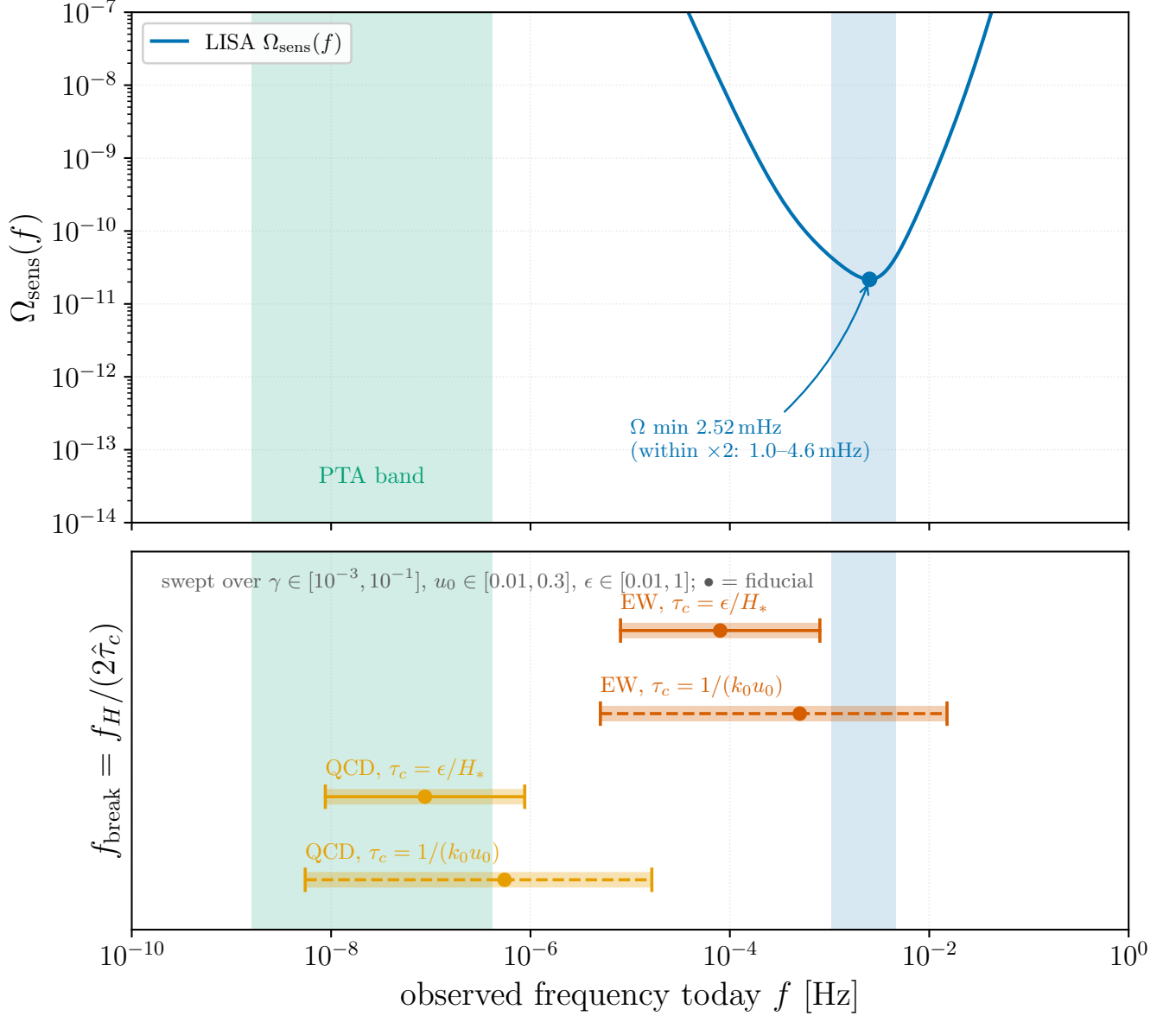
FIG. 17. Where the break falls relative to the observing bands. Top : the LISA energy-density sensitivity \Omega_{\text{sens}}(f) from the SciRD analytic noise model, with its minimum at 2.52 \text{ mHz} and the factor-of-two window shaded, and the pulsar-timing band. Bottom : f_{\text{break}} swept over the parameter ranges of Table VI for the two epochs and the two lifetime closures. The bands are two to three decades wide, which is the point: the break’s position relative to each instrument is robust where its value is not. Generated by Notebooks/k_break_frequency.py .
