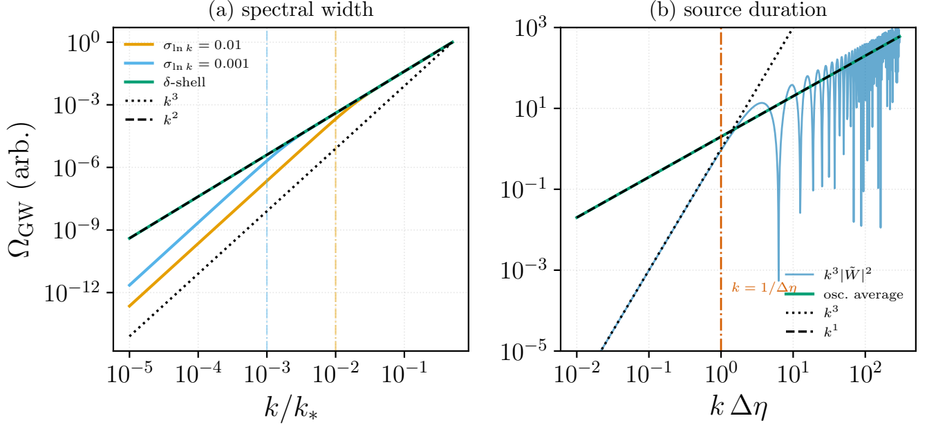
FIG. 11. Independent reproduction of the two exceptions to the universal k^3 infrared theorem of [9], computed from Eqs. (39) and (40) with no input from the kernels of this paper. (a) Shells of log-width \sigma_{\ln k} = 10^{-2} and 10^{-3} (dash-dotted verticals mark k = \sigma ) against an exact \delta -shell: the finite-width curves follow k^3 for k \ll \sigma and k^2 in the band \sigma \ll k \ll k_* , while the \delta -shell follows k^2 throughout, having no lower scale. (b) Finite emission window \Delta\eta : the spectrum follows k^3 below k = 1/\Delta\eta and, once the \sin^2 oscillations are averaged, k^1 above. Measured slopes are 3.000/2.000 and 2.999/1.000 respectively. Generated by Notebooks/cai_pi_sasaki_reproduction.py.
