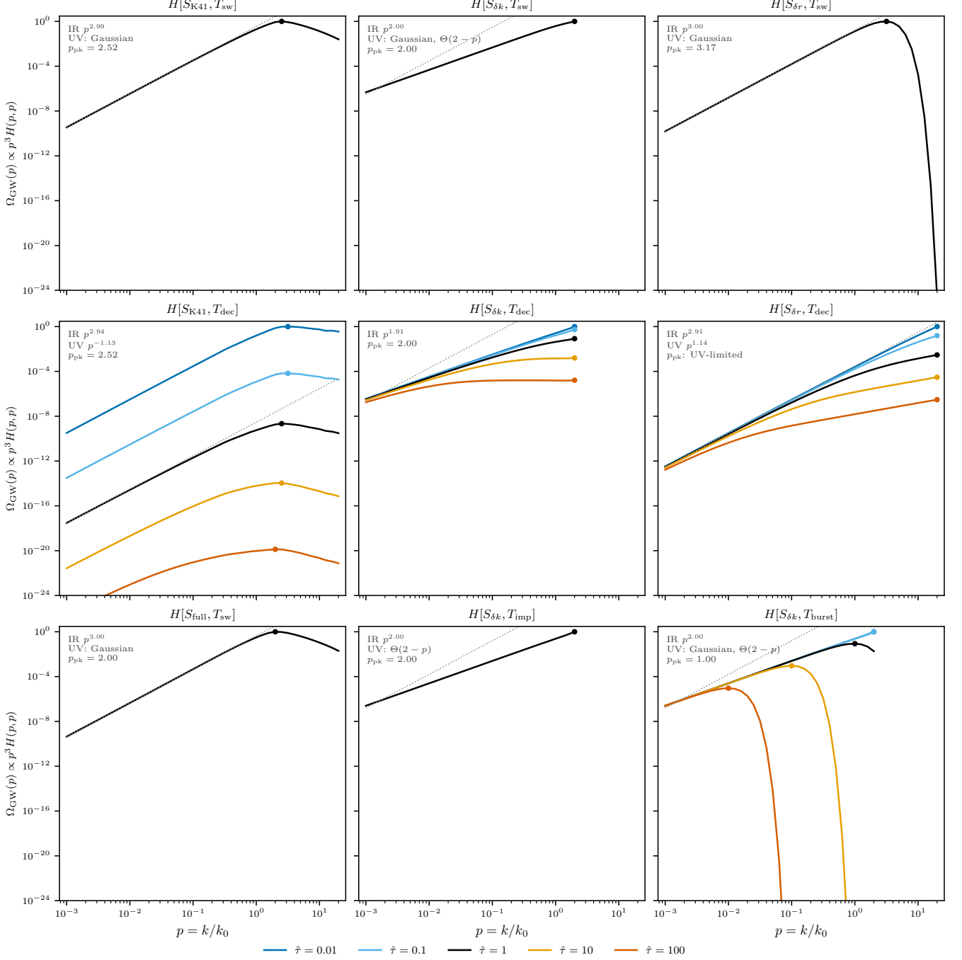
FIG. 17. The nine kernels of Table I at matched parameters, \Omega_{\text{GW}}(p) \propto p^3 H[S, T](p, p) on the sound-cone diagonal, p = k/k_0 , at R = 10^4 (and R_{\text{IR}} = 10^2 with a Batchelor infrared band for S_{\text{full}} ). Rows group the temporal model: sweeping (top), decaying (middle), and the full-spectrum, impulsive and burst cases (bottom). Curves are indexed by \hat{\tau} = \tau_c k_0 of Eq. (93); stationary and time-independent kernels carry the single reference line \hat{\tau} = 1 (equivalently M = \sqrt{2\pi} = 2.51 for the sweeping panels), the time-dependent ones the five values \hat{\tau} = 0.01, 0.1, 1, 10, 100 (equivalently M = 251, 25.1, 2.51, 0.251, 0.0251 ; the small- \hat{\tau} members are formal extrapolations past the luminal limit, retained as in Fig. 1 to expose the scaling). Each panel is normalised by its own maximum over all its curves, since the boxed kernels drop different dimensional prefactors and absolute amplitudes are not comparable between panels; within a panel the \hat{\tau} dependence of the amplitude is preserved. All nine panels share identical axes, set from the data so that the peak of every curve is on scale: the floor lies four decades below the faintest peak (the \hat{\tau} = 100 member of H[S_{K41}, T_{\text{dec}}] , suppressed as M^4 by Eq. (37)), which costs 24 decades of ordinate. The deep dives of the Gaussian-cutoff kernels leave the frame by design and carry no information: the \hat{\tau} = 100 burst reaches 10^{-277} before the triangle inequality terminates it. Dots mark peaks, the dotted grey line is the causal p^3 reference, and the annotations give the measured infrared slope, the ultraviolet behaviour and the peak of the \hat{\tau} = 1 curve. Generated by Notebooks/kernel.comparison.grid.py .
