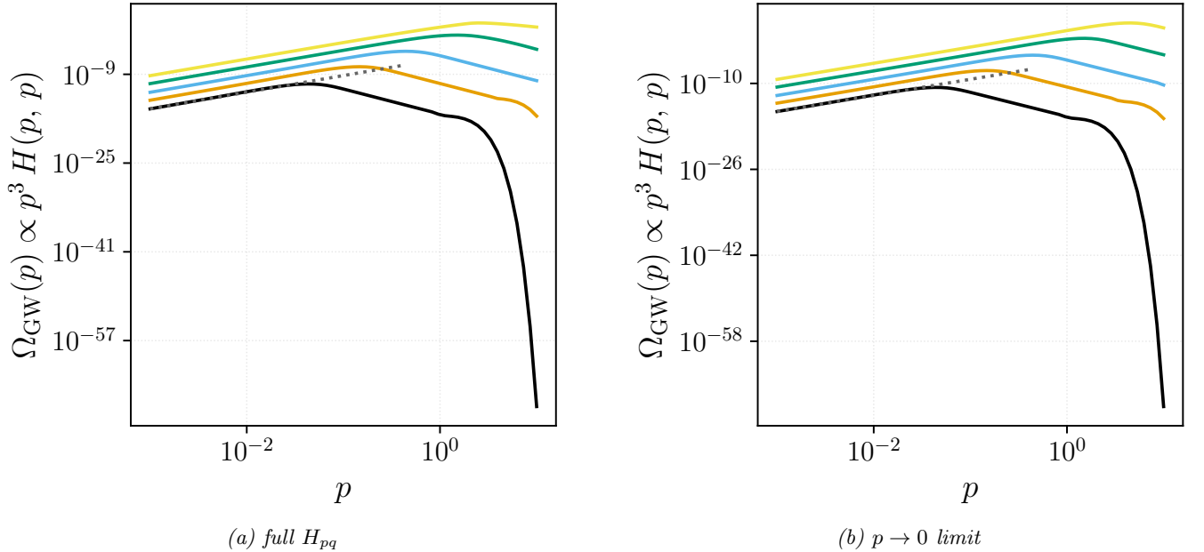
FIG. 14. Kraichnan decorrelation + Kolmogorov spectrum. Five curves per panel correspond to M = 0.03, 0.1, 0.3, 1.0, 3.0 at R = 10^4 . Panel (a) is the full numerical H_{pq} (Sec. II); panel (b) is the aeroacoustic p \rightarrow 0 limit (Kahniashvili et al. 2008). Both give the universal IR slope \Omega_{\text{GW}} \propto p^3 .
