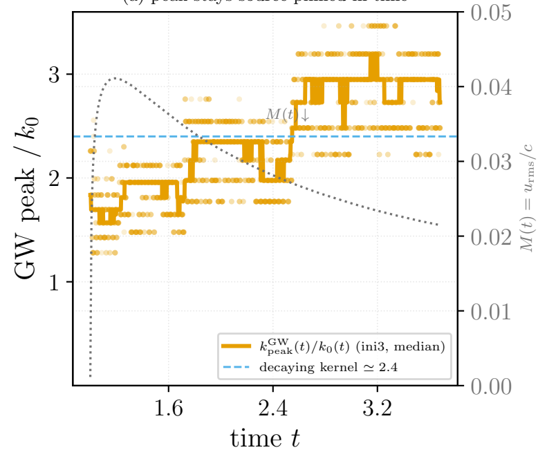
(a) peak stays source-pinned in time
