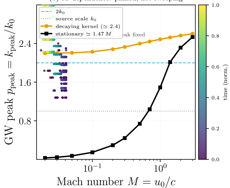
(b) M -dependence: pinned, not sweeping
