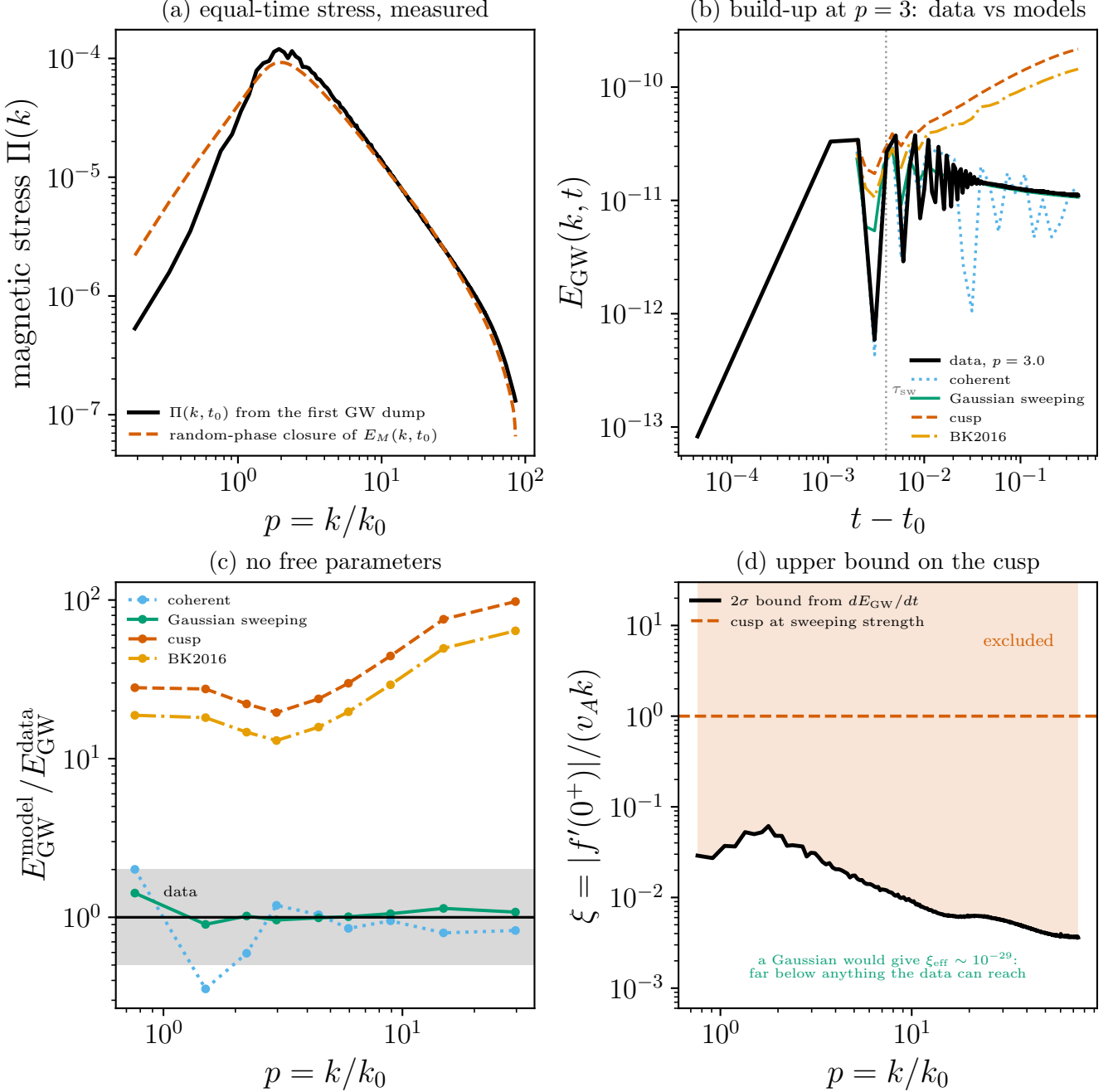
FIG. 6. Parameter-free forward models of run ini2 's GW spectrum from its own measured magnetic stress. Cuspless correlators reproduce the data; cusped ones overpredict by one to two orders of magnitude.
