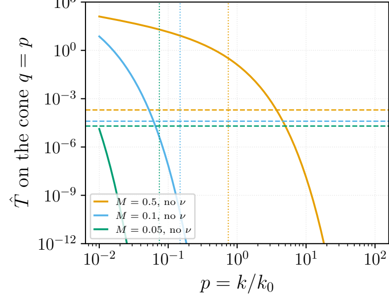
(a) Gaussian cutoff vs viscous floor 4M/R (b) crossover vs the sweeping peak
