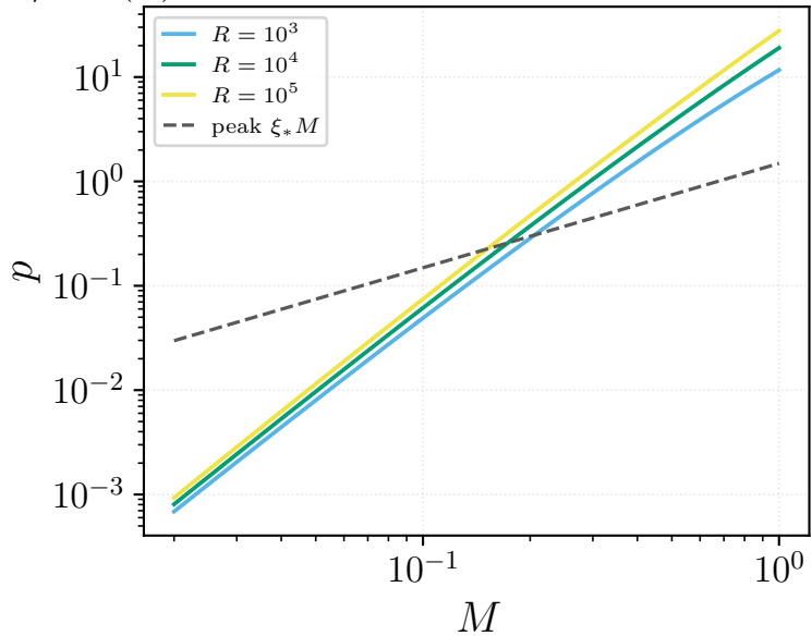
(a) Gaussian cutoff vs viscous floor 4M/R (b) crossover vs the sweeping peak
