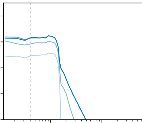
noh1 (nonhelical)
