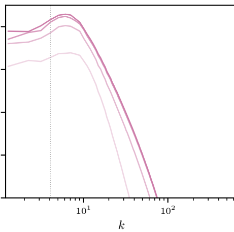
ac2 (acoustic)
