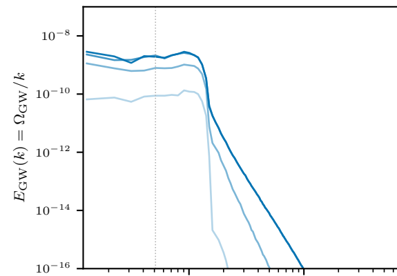
hel4 (helical)
