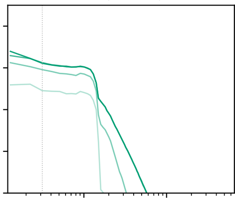
ac3 (acoustic)
