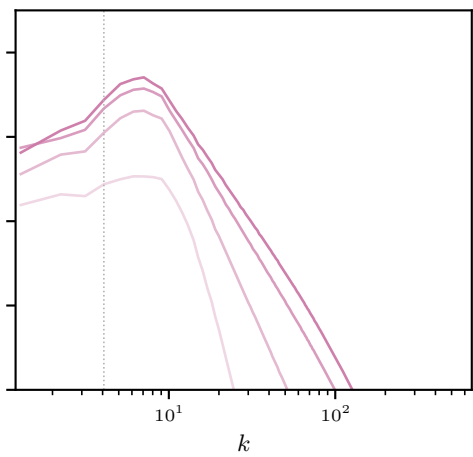
ac3 (acoustic)
