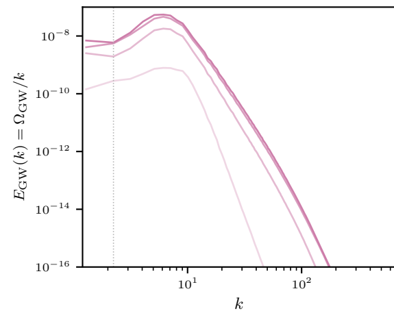
ac1 (acoustic)
