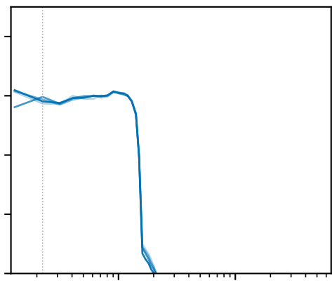
noh2 (nonhelical)
