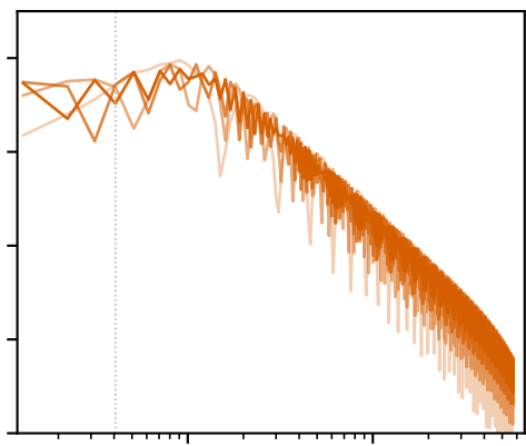
hel3 (helical)
