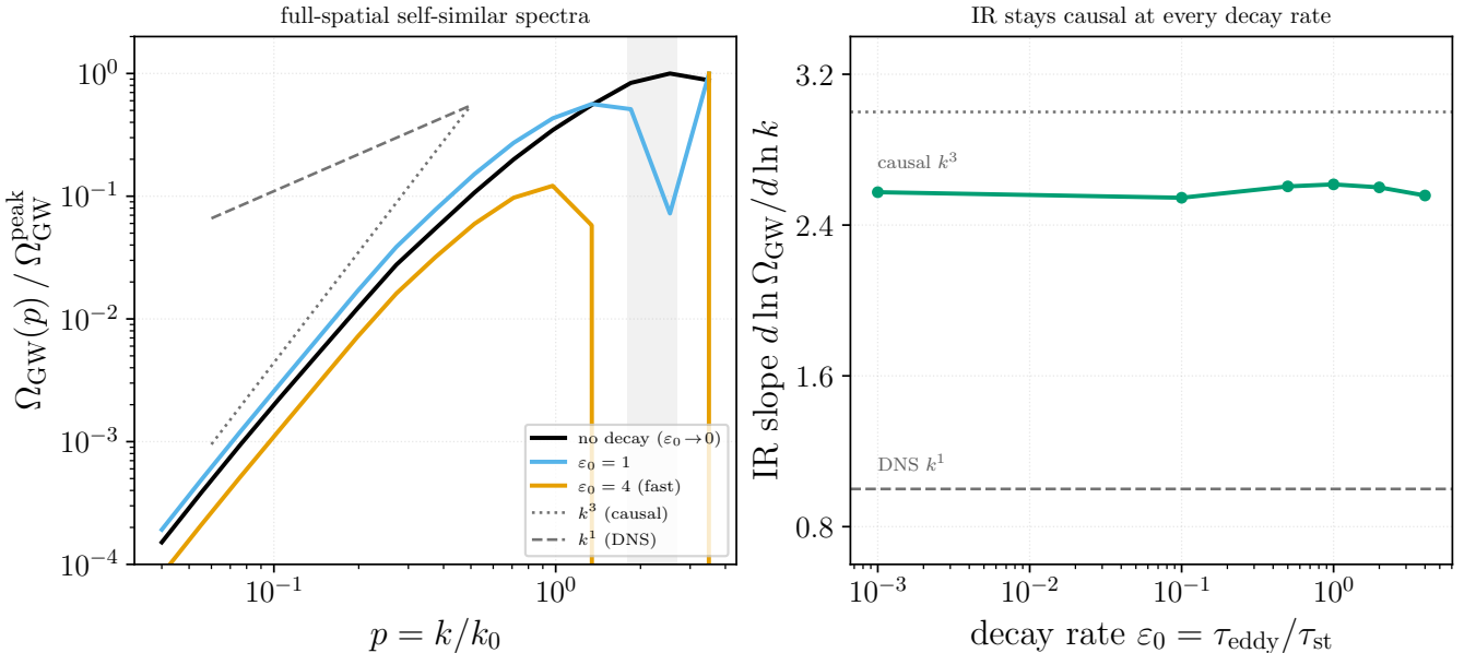
FIG. 9. The finite duration of a decaying source does not flatten the infrared. Left : GW spectra from the first-principles full-spatial self-similar kernel ( T_{\text{em}} = 40 \tau_{e0} , M = 1 ) at three decay rates; the infrared slopes overlap on the causal k^3 guide (dotted) rather than the k^1 guide (dashed), and share the source-scale peak (shaded). Right : the infrared slope versus the decay rate \varepsilon_0 = \tau_{\text{eddy}}/\tau_{\text{st}} stays at the causal value ( \simeq 2.5 –3) for every \varepsilon_0 , never approaching the simulated k^1 ; the physically realised self-similar decay sits at \varepsilon_0 \sim 1 . Generated by Notebooks/fullspatial_selfsimilar_exact.py .
