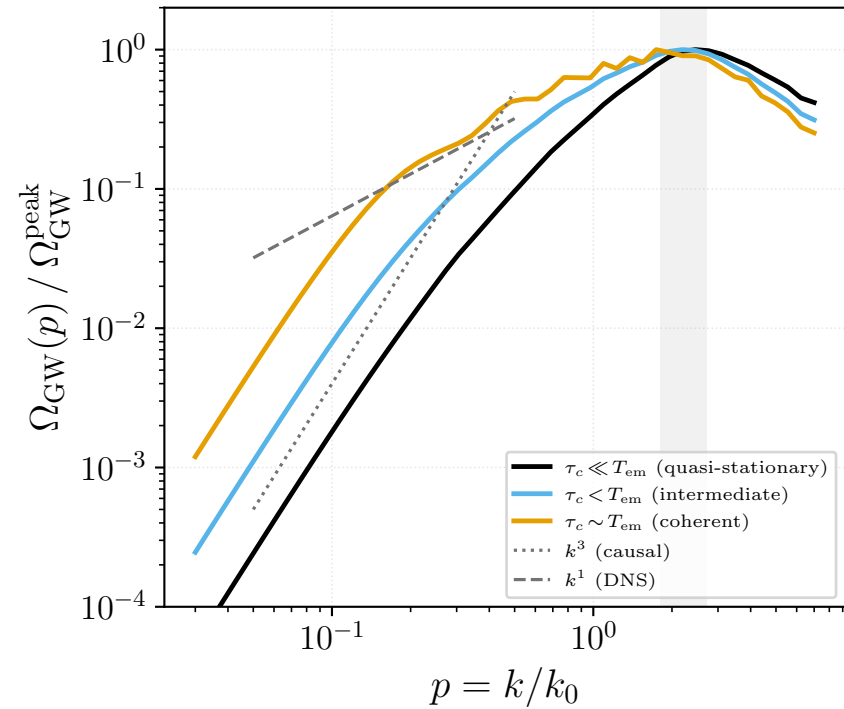
full-spatial spectrum, T_{\text{em}} = 20 \tau_{e0}
