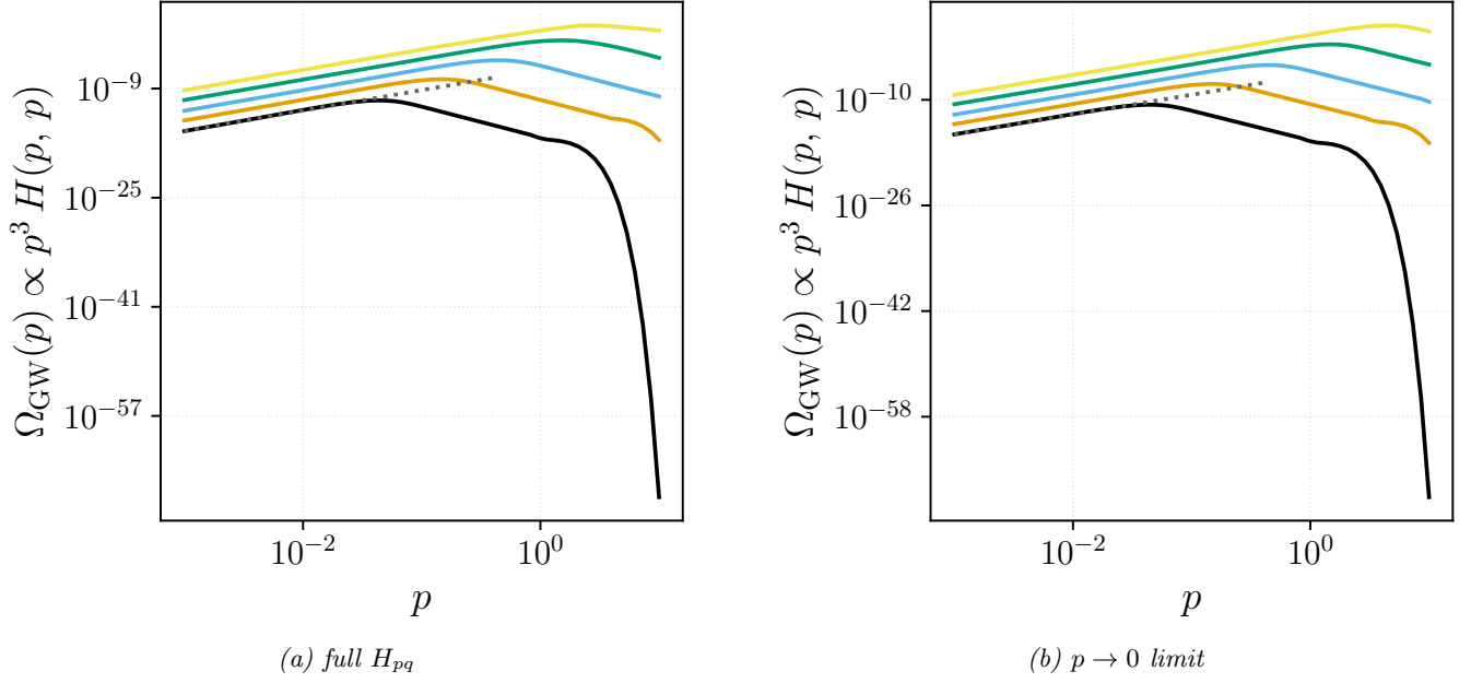
FIG. 23. Kraichnan decorrelation + Kolmogorov spectrum. Five curves per panel correspond to M = 0.03, 0.1, 0.3, 1.0, 3.0 at R = 10^4 . Panel (a) is the full numerical H_{pq} (Sec. III); panel (b) is the aeroacoustic p \rightarrow 0 limit (Kahniashvili et al. 2008). Both give the universal IR slope \Omega_{\text{GW}} \propto p^3 .
