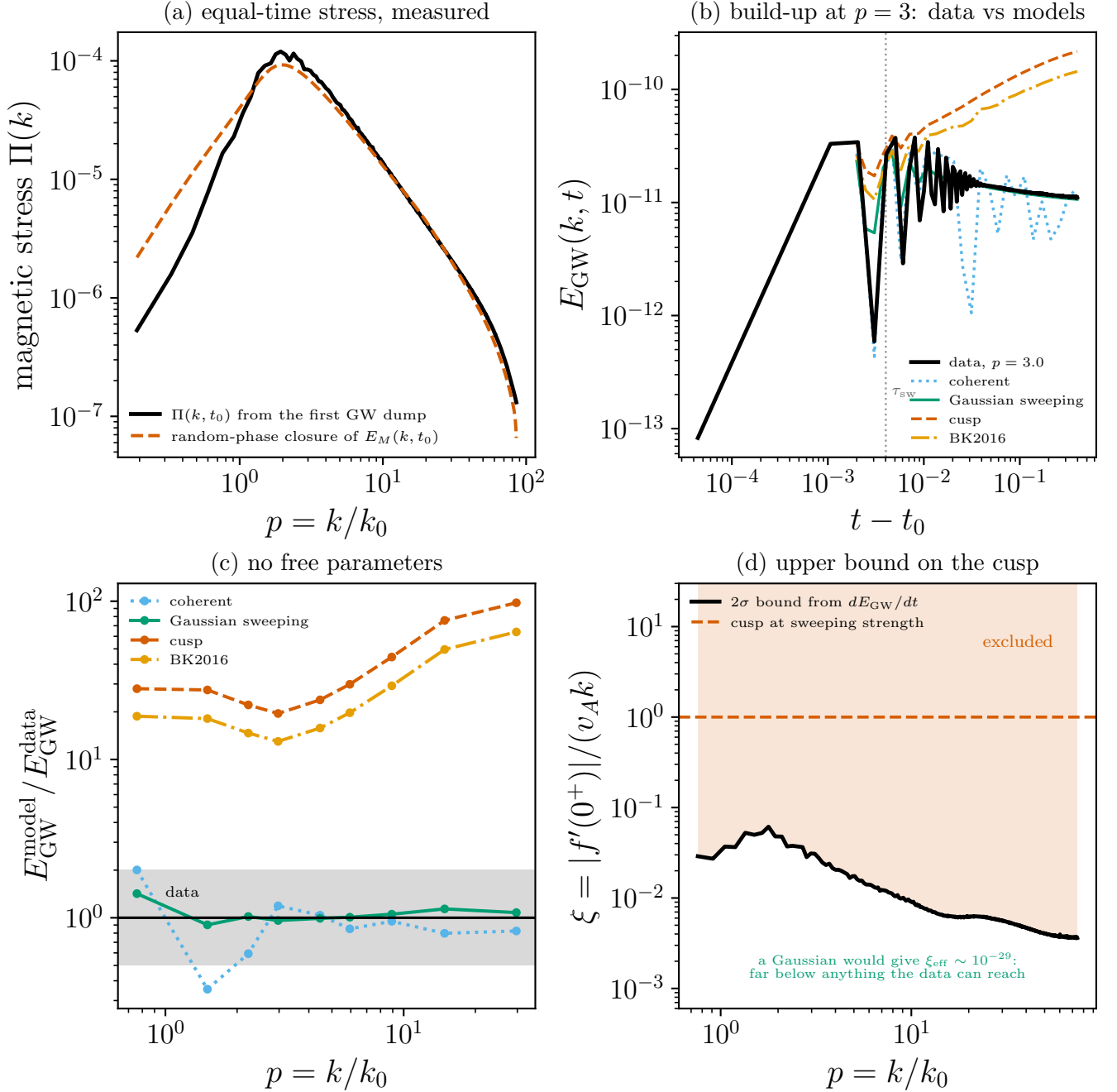
FIG. 6. Parameter-free forward models of run ini2's GW spectrum from its own measured magnetic stress. Cuspless correlators reproduce the data; cusped ones overpredict by one to two orders of magnitude.
