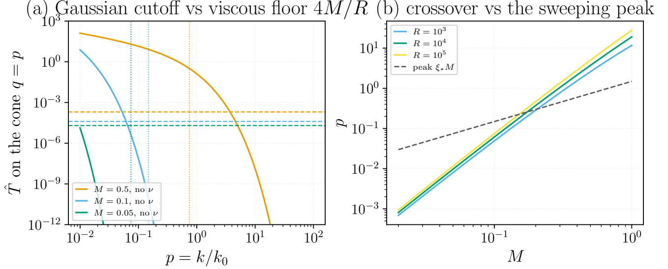
FIG. 20. The viscous cusp. (a) The two-leg sweeping factor on the cone q = p (solid) against the viscous floor 4M/R of Eq. (56) (dashed) at R = 10^4 ; dotted verticals mark the sweeping peak \xi_* M . The Gaussian is super-exponential in p^{2/3}/M^2 , so the constant floor overtakes it, and the more subsonic the flow the earlier. (b) The crossover against M for three Reynolds numbers, with the peak \xi_* M dashed: the floor emerges above the peak for M \gtrsim 0.3 and below it for M \lesssim 0.1 . Temporal factor only — the full two-wavevector kernel is not evaluated here. Generated by Notebooks/viscous_cusp_floor.py .
