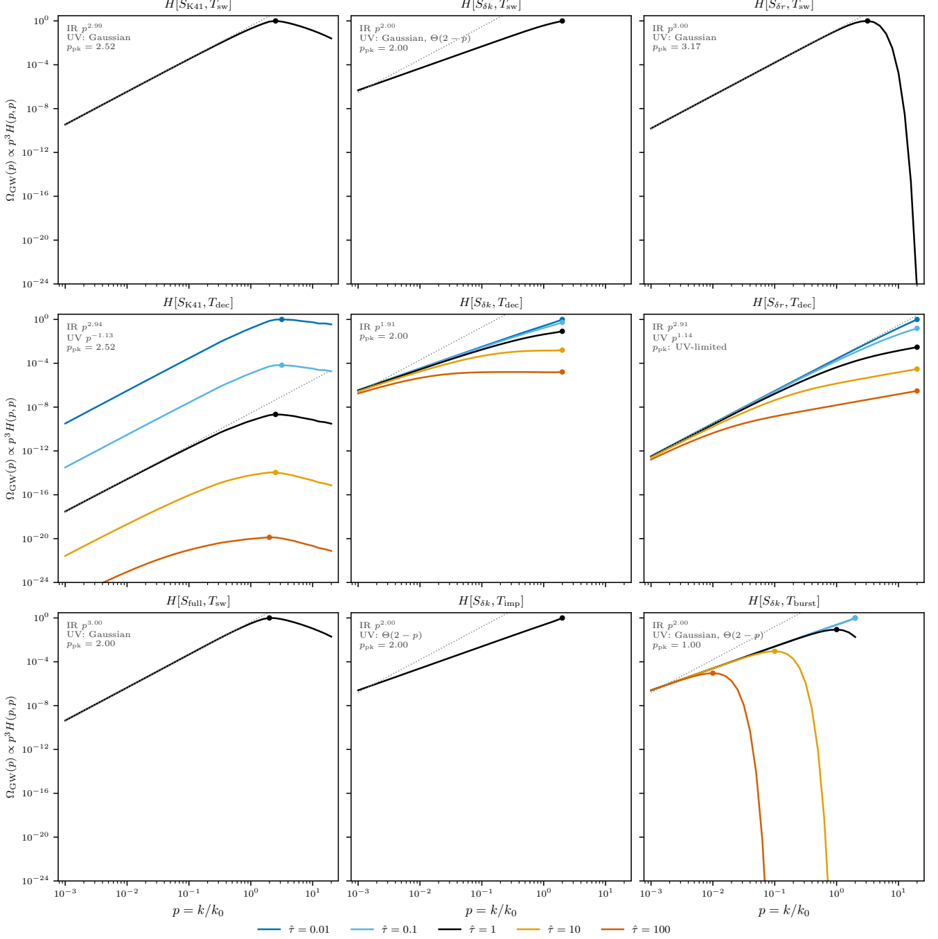
FIG. 22. The nine kernels of Table I at matched parameters, \Omega_{\text{GW}}(p) \propto p^3 H[S, T](p, p) on the sound-cone diagonal, p = k/k_0 , at R = 10^4 (and R_{\text{IR}} = 10^2 with a Batchelor infrared band for S_{\text{full}} ). Rows group the temporal model: sweeping (top), decaying (middle), and the full-spectrum, impulsive and burst cases (bottom). Curves are indexed by \hat{\tau} = \tau_c k_0 of Eq. (H2); stationary and time-independent kernels carry the single reference line \hat{\tau} = 1 (equivalently M = \sqrt{2\pi} = 2.51 for the sweeping panels), the time-dependent ones the five values \hat{\tau} = 0.01, 0.1, 1, 10, 100 (equivalently M = 251, 25.1, 2.51, 0.251, 0.0251 ; the small- \hat{\tau} members are formal extrapolations past the luminal limit, retained as in Fig. 1 to expose the scaling). Each panel is normalised by its own maximum over all its curves, since the boxed kernels drop different dimensional prefactors and absolute amplitudes are not comparable between panels; within a panel the \hat{\tau} dependence of the amplitude is preserved. All nine panels share identical axes, set from the data so that the peak of every curve is on scale: the floor lies four decades below the faintest peak (the \hat{\tau} = 100 member of H[S_{K41}, T_{\text{dec}}] , suppressed as M^4 by Eq. (38)), which costs 24 decades of ordinate. The deep dives of the Gaussian-cutoff kernels leave the frame by design and carry no information: the \hat{\tau} = 100 burst reaches 10^{-277} before the triangle inequality terminates it. Dots mark peaks, the dotted grey line is the causal p^3 reference, and the annotations give the measured infrared slope, the ultraviolet behaviour and the peak of the \hat{\tau} = 1 curve. Generated by Notebooks/kernel.comparison.grid.py .
