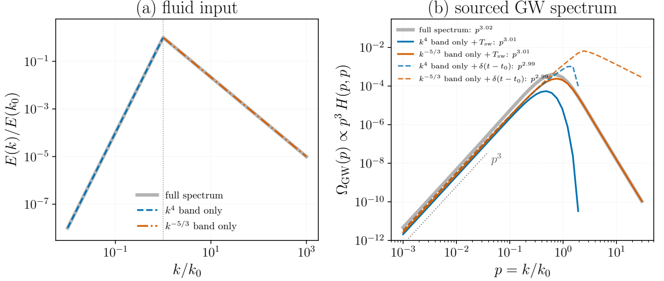
FIG. 15. Band-split test of the white-noise-floor hypothesis. (a) The three fluid inputs fed to the kernel: the full spectrum of Eq. (25) (grey), its Batchelor band E \propto k^4 alone (blue, dashed) and its Kolmogorov range E \propto k^{-5/3} alone (orange, dash-dotted), obtained by masking the shape factor S(k) = A(k)/A_{\text{Kol}}(k) on one side of k_0 (dotted vertical line). (b) The gravitational-wave spectra \Omega_{\text{GW}}(p) \propto p^3 H_{ijij}(p, p; M, R) they source on the sound-cone diagonal q = p , with the infrared log-log slopes fitted over 2 \times 10^{-3} \leq p \leq 2 \times 10^{-2} quoted in the legend; the dotted guide is p^3 . All are causal to better than 2% in the exponent, including the inertial-range-only run, whose input has no infrared power at all. The Batchelor-only spectrum ends at p = 2 , the kinematic limit of a convolution of two modes with k < k_0 . The two dashed curves repeat the single-band runs with the temporal factor removed entirely—evaluated at q = 0 rather than on the diagonal q = p , so that the Gaussian sweeping factor and its erfc in Eq. (23) are both unity and the source carries no decorrelation and no time dependence at all [the impulsive limit, Eq. (B105)]. The spatial integral is otherwise identical, so each solid/dashed pair isolates what the temporal model does and does not control. Parameters: M = 0.5 , R = (k_d/k_0)^{4/3} = 10^4 , R_{\text{IR}} = k_0/k_{\text{IR}} = 10^2 , Batchelor infrared slope s = 4 . Both panels are dimensionless and the vertical offset between them carries no physical meaning. Produced by Notebooks/band_split_gw.py .
