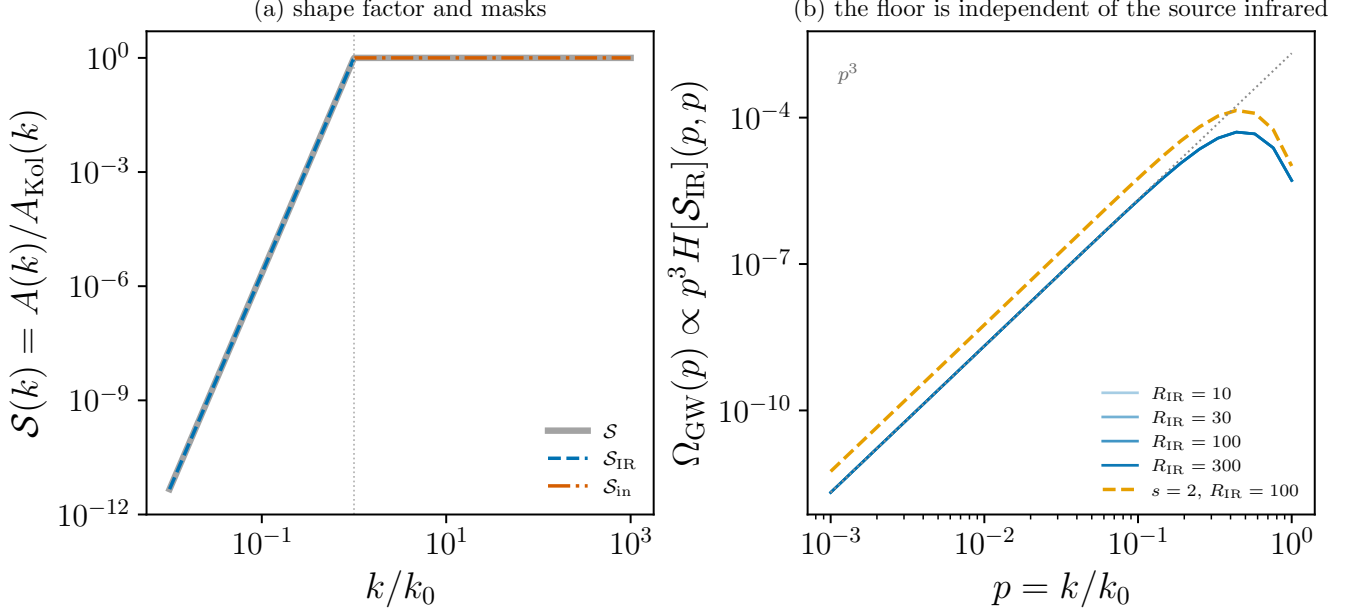
FIG. 17. The two ingredients of the band-split chain. (a) The shape factor \mathcal{S} of Eq. (B116) and its masks \mathcal{S}_{\text{IR}}, \mathcal{S}_{\text{in}} of Eq. (B117). The masks have disjoint support and sum to \mathcal{S} , so each traces it exactly on its own side of k_0 (dotted vertical); this is what makes the decomposition Eq. (B120) exact rather than approximate. (b) Eq. (B121) made visible: the infrared band alone, \Omega_{\text{GW}} \propto p^3 H[\mathcal{S}_{\text{IR}}](p, p) , at four infrared bandwidths R_{\text{IR}} = 10, 30, 100, 300 and at two infrared slopes s = 4 (Batchelor) and s = 2 (Saffman), with M = 0.5, R = 10^4 . The four bandwidth curves are drawn separately but are not distinguishable: they agree to 0.31% at p = 5 \times 10^{-3} despite spanning 1.5 decades of R_{\text{IR}} , because the floor P_T(0) = \int d^3 q P_M(q)^2 is fixed by the modes at the top of the band and is blind to how far the band extends. Changing the infrared slope itself moves the amplitude by only 2.71 and leaves the exponent at 3.005 against 3.001, although the two inputs differ by four decades at the bottom of the band. Dotted guide: p^3 . Produced by Notebooks/band_split_masks.py .
