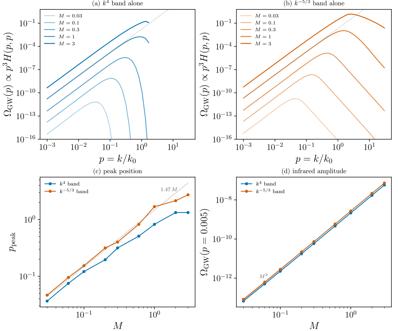
FIG. 16. Mach dependence of the band-split spectra, at R = 10^4 , R_{\text{IR}} = 10^2 , Kraichnan sweeping on the diagonal q = p . (a), (b) \Omega_{\text{GW}}(p) from the Batchelor k^4 band alone and from the Kolmogorov k^{-5/3} band alone, at M = 0.03, 0.1, 0.3, 1, 3 (increasing shade); dotted line p^3 . The infrared exponent is M -independent for both bands; the amplitude and the peak are not. (c) Peak position against M , with the 1.49 M sweeping law of Eq. (31) dotted. The inertial band reproduces it; the Batchelor band tracks a slightly lower 1.1 M and saturates above M \simeq 1 , where the sweeping scale meets the kinematic ceiling p \leq 2 that bounds a convolution of two modes with k < k_0 . (d) Infrared amplitude at p = 5 \times 10^{-3} against M , with the M^3 prefactor dotted; both bands follow it to 13% and 19% over two decades of M . Produced by Notebooks/band_split_mach.py .
