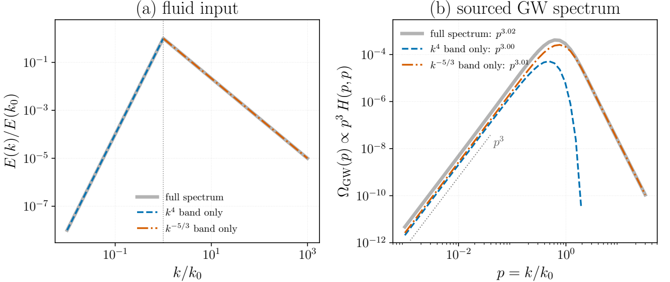
FIG. 13. Band-split test of the white-noise-floor hypothesis. (a) The three fluid inputs fed to the kernel: the full spectrum of Eq. (24) (grey), its Batchelor band E \propto k^4 alone (blue, dashed) and its Kolmogorov range E \propto k^{-5/3} alone (orange, dash-dotted), obtained by masking the shape factor S(k) = A(k)/A_{\text{Kol}}(k) on one side of k_0 (dotted vertical line). (b) The gravitational-wave spectra \Omega_{\text{GW}}(p) \propto p^3 H_{ijij}(p, p; M, R) they source on the sound-cone diagonal q = p , with the infrared log-log slopes fitted over 2 \times 10^{-3} \leq p \leq 2 \times 10^{-2} quoted in the legend; the dotted guide is p^3 . All three are causal to better than 2% in the exponent, including the inertial-range-only run, whose input has no infrared power at all. The Batchelor-only spectrum ends at p = 2 , the kinematic limit of a convolution of two modes with k < k_0 . Parameters: M = 0.5 , R = (k_d/k_0)^{4/3} = 10^4 , R_{\text{IR}} = k_0/k_{\text{IR}} = 10^2 , Batchelor infrared slope s = 4 . Both panels are dimensionless and the vertical offset between them carries no physical meaning. Produced by Notebooks/band_split_gw.py .
