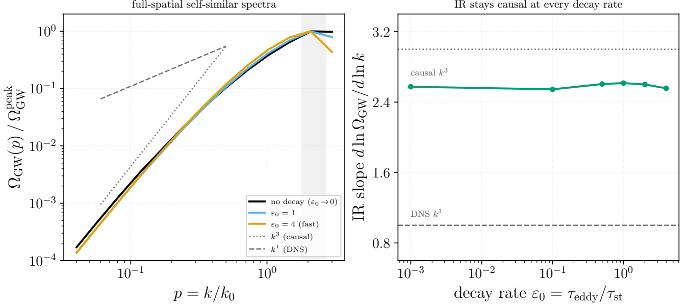
FIG. 11. The finite duration of a decaying source does not flatten the infrared. Left : GW spectra from the first-principles full-spatial self-similar kernel ( T_{\text{em}} = 40 \tau_{e0} , M = 1 ) at three decay rates; the infrared slopes overlap on the causal k^3 guide (dotted) rather than the k^1 guide (dashed), and share the source-scale peak (shaded). Right : the infrared slope versus the decay rate \varepsilon_0 = \tau_{\text{eddy}}/\tau_{\text{st}} stays at the causal value ( \simeq 2.5\text{--}3 ) for every \varepsilon_0 , never approaching the simulated k^1 ; the physically realised self-similar decay sits at \varepsilon_0 \sim 1 . Generated by Notebooks/fullspatial_selfsimilar_exact.py .
