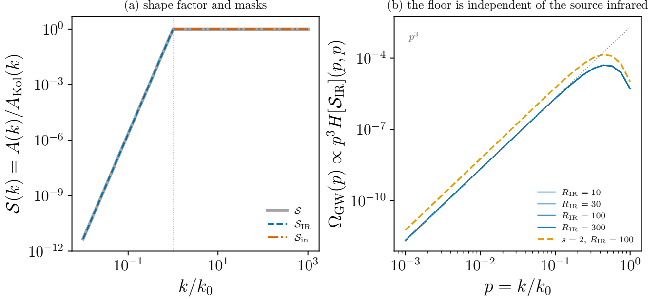
FIG. 19. The two ingredients of the band-split chain. (a) The shape factor S of Eq. (B116) and its masks S_{\text{IR}}, S_{\text{in}} of Eq. (B117). The masks have disjoint support and sum to S , so each traces it exactly on its own side of k_0 (dotted vertical); this is what makes the decomposition Eq. (B120) exact rather than approximate. (b) Eq. (B121) made visible: the infrared band alone, \Omega_{\text{GW}} \propto p^3 H[S_{\text{IR}}](p, p) , at four infrared bandwidths R_{\text{IR}} = 10, 30, 100, 300 and at two infrared slopes s = 4 (Batchelor) and s = 2 (Saffman), with M = 0.5 , R = 10^4 . The four bandwidth curves are drawn separately but are not distinguishable: they agree to 0.31% at p = 5 \times 10^{-3} despite spanning 1.5 decades of R_{\text{IR}} , because the floor P_T(0) = \int d^3 q P_M(q)^2 is fixed by the modes at the top of the band and is blind to how far the band extends. Changing the infrared slope itself moves the amplitude by only 2.71 and leaves the exponent at 3.005 against 3.001, although the two inputs differ by four decades at the bottom of the band. Dotted guide: p^3 . Produced by Notebooks/band_split_masks.py .
