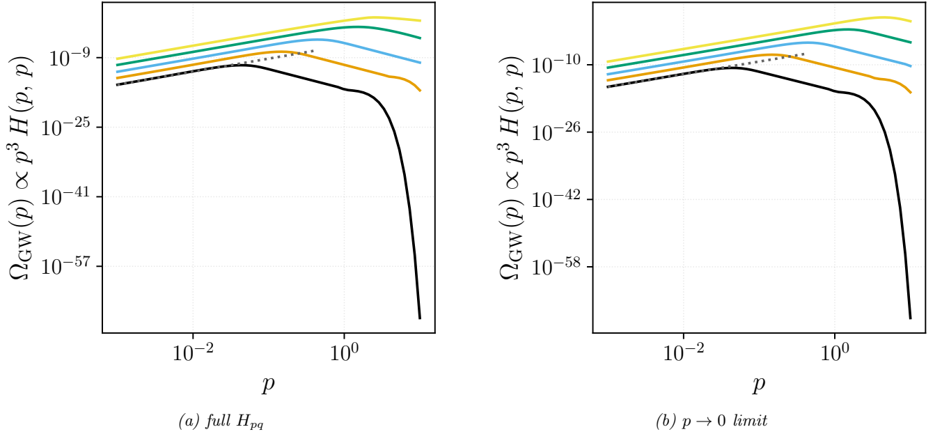
FIG. 15. Kraichnan decorrelation + Kolmogorov spectrum. Five curves per panel correspond to M = 0.03, 0.1, 0.3, 1.0, 3.0 at R = 10^4 . Panel (a) is the full numerical H_{pq} (Sec. II); panel (b) is the aeroacoustic p \rightarrow 0 limit (Kahnishvili et al. 2008). Both give the universal IR slope \Omega_{\text{GW}} \propto p^3 .
