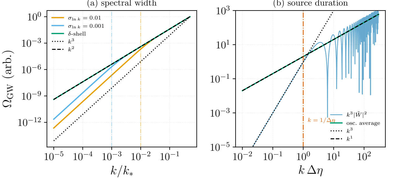
FIG. 12. Independent reproduction of the two exceptions to the universal k^3 infrared theorem of [9], computed from Eqs. (44) and (45) with no input from the kernels of this paper. (a) Shells of log-width \sigma_{\ln k} = 10^{-2} and 10^{-3} (dash-dotted verticals mark k = \sigma ) against an exact \delta -shell: the finite-width curves follow k^3 for k \ll \sigma and k^2 in the band \sigma \ll k \ll k_* , while the \delta -shell follows k^2 throughout, having no lower scale. (b) Finite emission window \Delta\eta : the spectrum follows k^3 below k = 1/\Delta\eta and, once the \sin^2 oscillations are averaged, k^1 above. Measured slopes are 3.000/2.000 and 2.999/1.000 respectively. Generated by Notebooks/cai_pi_sasaki_reproduction.py .
