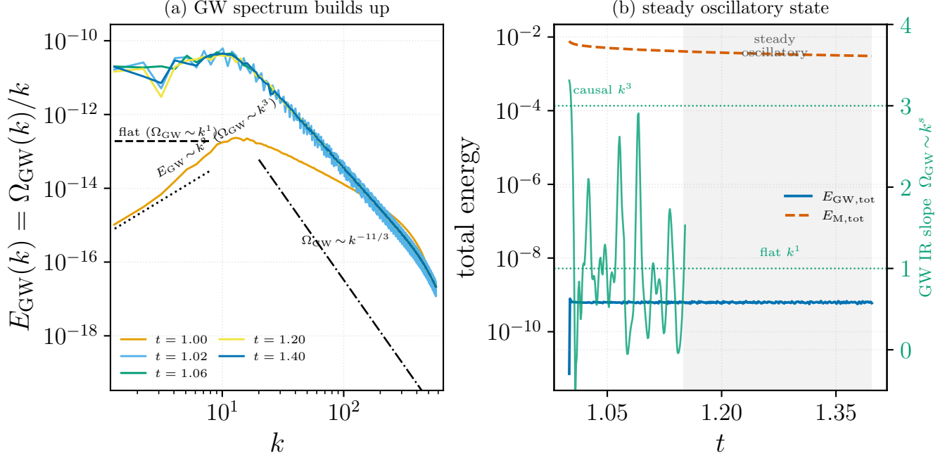
FIG. 10. Time-series reanalysis of the Roper Pol et al. [6] run ini2 (public Pencil Code spectra, Zenodo 10.5281/zenodo.3692072), the run of their Fig. 1. (a) The GW energy spectrum E_{\text{GW}} = \Omega_{\text{GW}}/k at successive times: at switch-on ( t \simeq 1.0 ) the infrared follows the causal E_{\text{GW}} \sim k^2 ( \Omega_{\text{GW}} \sim k^3 ) and within \Delta t \sim 0.02 saturates to the flat plateau ( \Omega_{\text{GW}} \sim k^1 ) of their Fig. 1. (b) Total energies versus time: the GW energy rises while the source acts, then fluctuates about a steady mean (grey band; the “steady oscillatory state”), while the magnetic energy keeps decaying; the right axis (green) shows the measured GW infrared slope crossing from the causal k^3 to the saturated k^1 . Generated by Notebooks/roperpol_timeseries.py , which auto-downloads the data.
