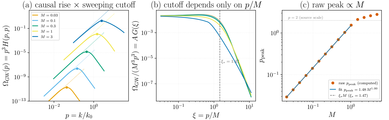
FIG. 3. Why the stationary GW spectrum peaks at p \simeq 1.47M rather than at the source scale p \sim 2 , computed from \Omega_{\text{GW}}(p) = p^3 H_{ijij}(p, p; M, R) [Eq. (21), R = 10^4 ]. (a) Each spectrum (solid) follows its causal infrared asymptote A M^3 p^3 (dotted) and rolls over at the peak (dot) where the sweeping cutoff switches on. (b) Collapse: \Omega_{\text{GW}}/(M^3 p^3) versus \xi = p/M falls on a single curve AG(\xi) for every M , proving the cutoff depends only on p/M [Eq. (25)]; the universal peak position is \xi_* = 1.47 . (c) Peak location read directly from each computed spectrum (points) versus M : a power law p_{\text{peak}} = 1.48 M^{1.00} (line) [Eq. (27)], coincident with \xi_* M (dashed), that bends below it toward the p = 2 source scale (dotted) only at transonic M . Generated by Notebooks/stationary_peak_analysis.py .
