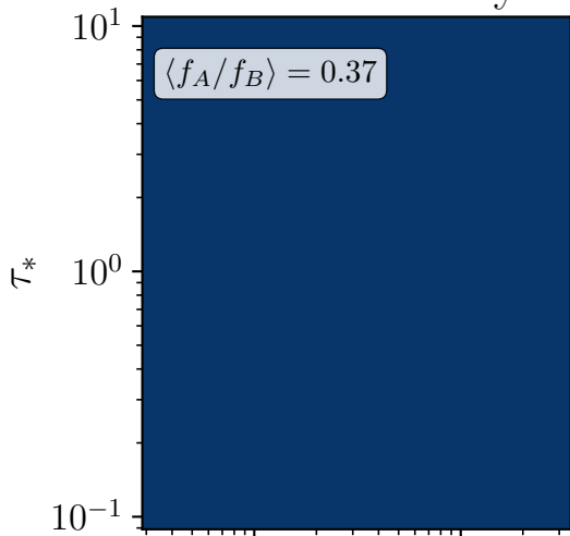
nonhelical MHD
