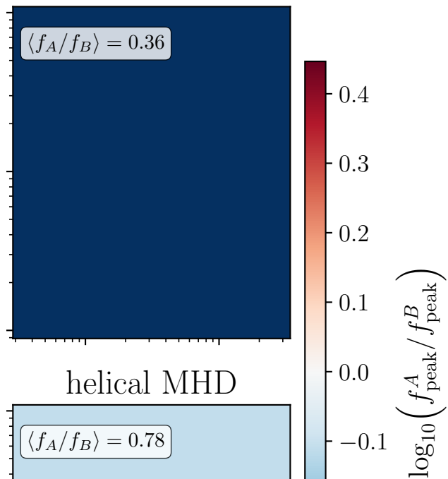
HD Saffman
