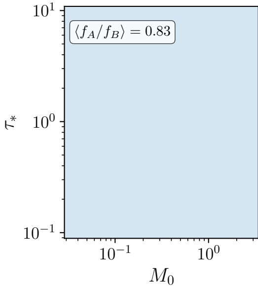
nonhelical MHD
