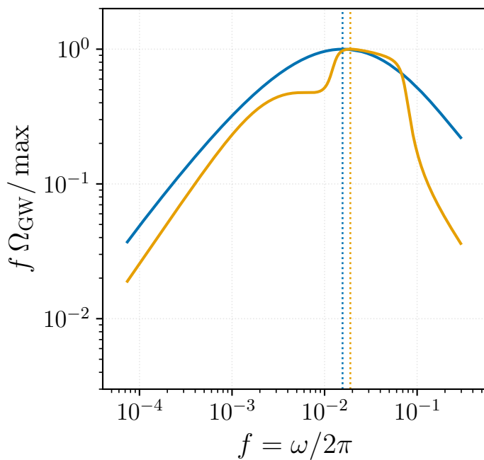
nonhelical MHD
