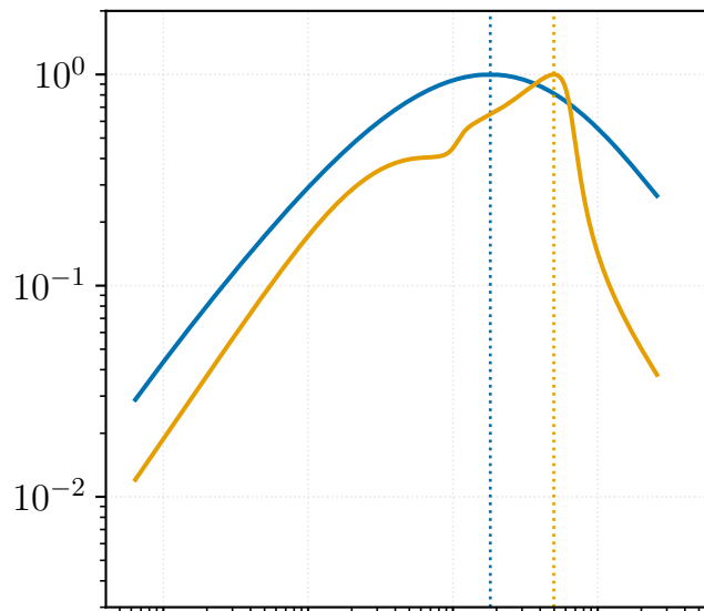
HD Saffman
