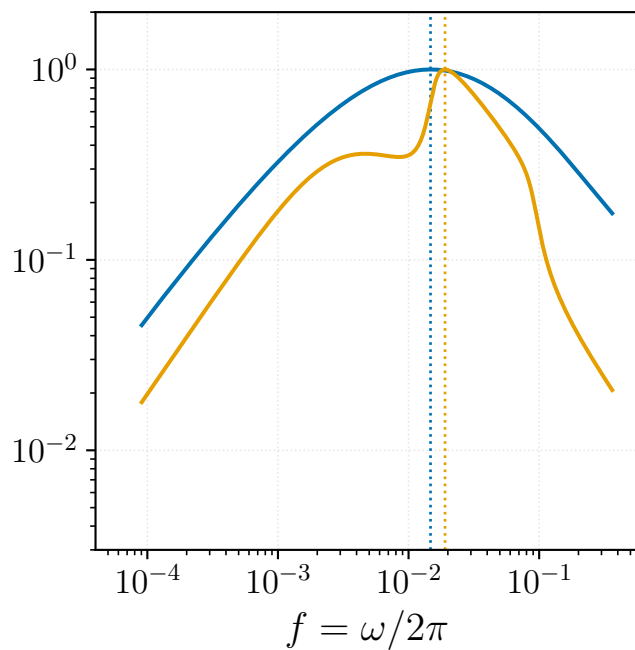
helical MHD
