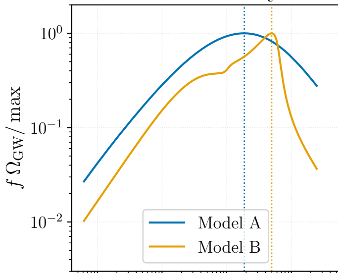
HD Loitsiansky
