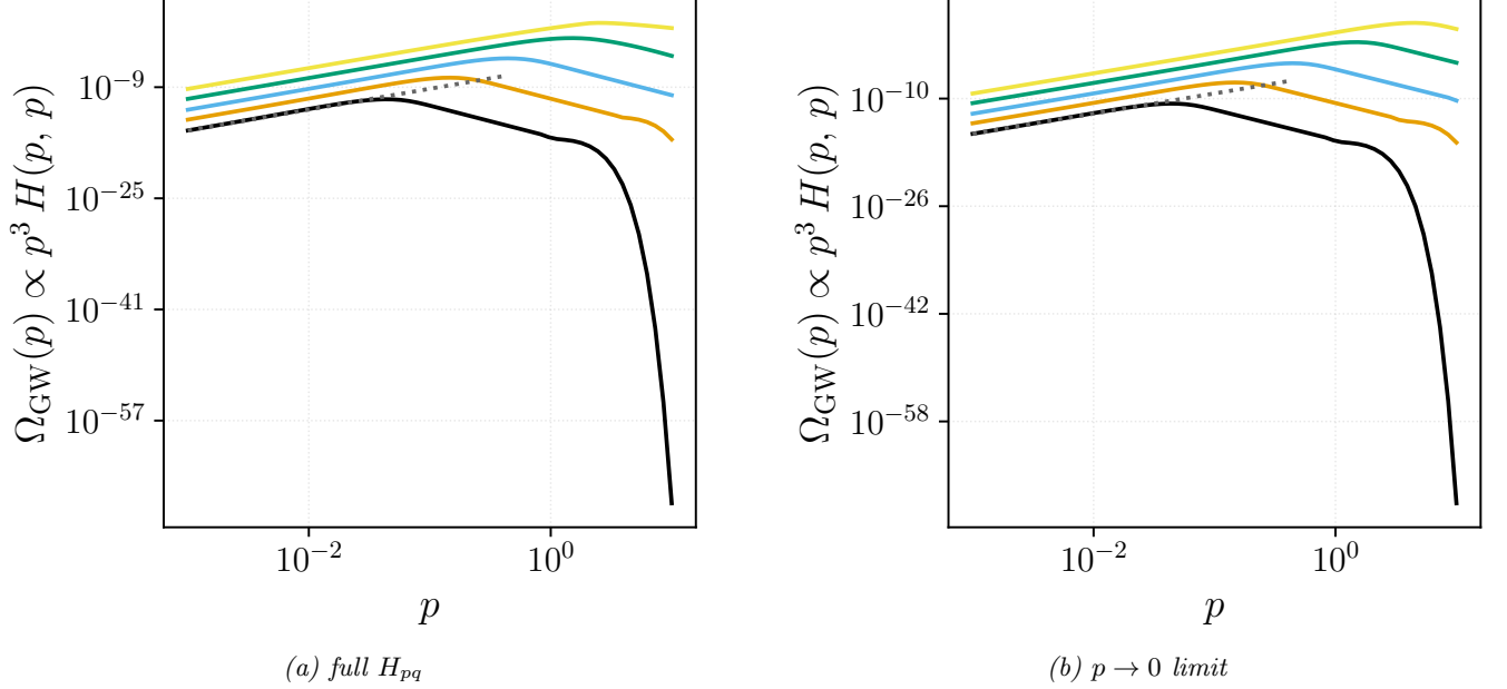
FIG. 10. Kraichnan decorrelation + Kolmogorov spectrum. Five curves per panel correspond to M = 0.03, 0.1, 0.3, 1.0, 3.0 at R = 10^4 . Panel (a) is the full numerical H_{pq} (Sec. II); panel (b) is the aeroacoustic p \rightarrow 0 limit (Kahniashvili et al. 2008). Both give the universal IR slope \Omega_{\text{GW}} \propto p^3 .
