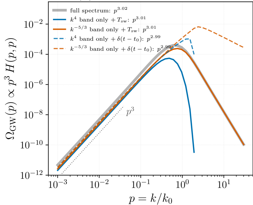
(b) sourced GW spectrum
