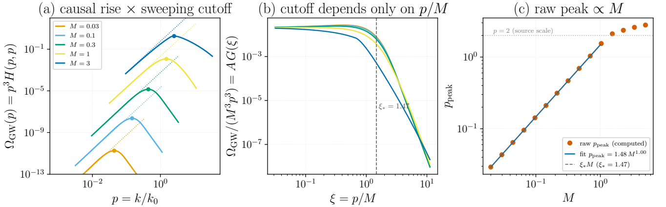
FIG. 3. Why the stationary GW spectrum peaks at p \simeq 1.47 M rather than at the source scale p \sim 2 , computed from \Omega_{\text{GW}}(p) = p^3 H_{ijij}(p, p; M, R) [Eq. (23), R = 10^4 ]. (a) Each spectrum (solid) follows its causal infrared asymptote A M^3 p^3 (dotted) and rolls over at the peak (dot) where the sweeping cutoff switches on. (b) Collapse: \Omega_{\text{GW}}/(M^3 p^3) = H_{ijij}(p, p; M)/M^3 versus \xi = p/M falls on the single compensated kernel \tilde{H}_{ijij}(\xi) for every M , proving the cutoff depends only on p/M [Eq. (28)]; the universal peak position is \xi_* = 1.47 . (c) Peak location read directly from each computed spectrum (points) versus M : a power law p_{\text{peak}} = 1.48 M^{1.00} (line) [Eq. (31)], coincident with \xi_* M (dashed), that bends below it toward the p = 2 source scale (dotted) only as M \rightarrow 1 (the luminal limit; M > 1 is superluminal). Generated by Notebooks/stationary_peak_analysis.py .
