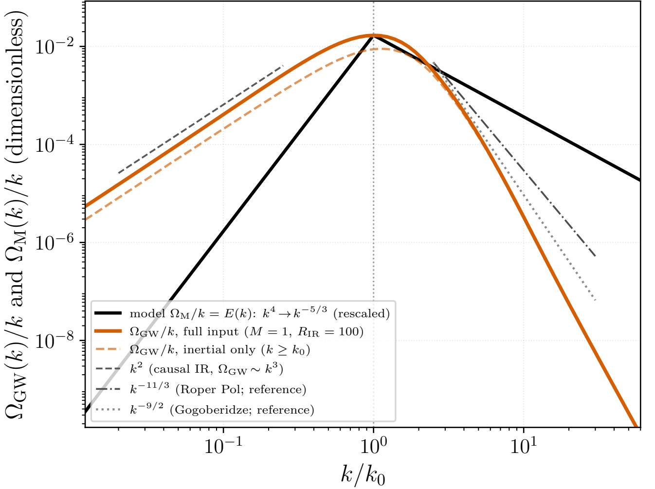
FIG. 2. Analytic spectra in the Roper Pol et al. [22] convention \Omega(k)/k = E(k) . Orange (solid): GW spectrum \Omega_{\text{GW}}(k)/k = p^2 H_{ijij}(p, p; M, R) [Eq. (23)] computed from a full fluid input spectrum—an infrared band E \propto k^4 ( k < k_0 ) joined to the Kolmogorov range E \propto k^{-5/3} ( k \geq k_0 ), Eq. (24)—fed into the Appendix-A kernel Eq. (19) through the shape factor S(k) = A/A_{\text{Kol}} ( M = 1 , R = 10^4 , infrared range R_{\text{IR}} = k_0/k_{\text{IR}} = 100 ). Orange (dashed): the same kernel restricted to the inertial range only ( R_{\text{IR}} = 1 , i.e. core Eq. (22))—the infrared band raises the amplitude near the peak but leaves the ultraviolet unchanged. Black: the full fluid input spectrum, rescaled to share the GW peak (the GW–fluid vertical offset is unphysical; only shapes compare). Grey dashed: the causal infrared guide k^2 ( \Omega_{\text{GW}} \sim k^3 ). Dash-dot/dotted: the k^{-11/3} (Roper Pol, run ini2) and k^{-9/2} (Gogoberidze) slopes reported in the literature, as references only—no simulation data points are plotted. At M = 1 the GW spectrum steepens past the peak to \simeq k^{-5.0} , steeper than both references, independently of the infrared treatment. Generated by Notebooks/roperpol_convention_spectra.py .
