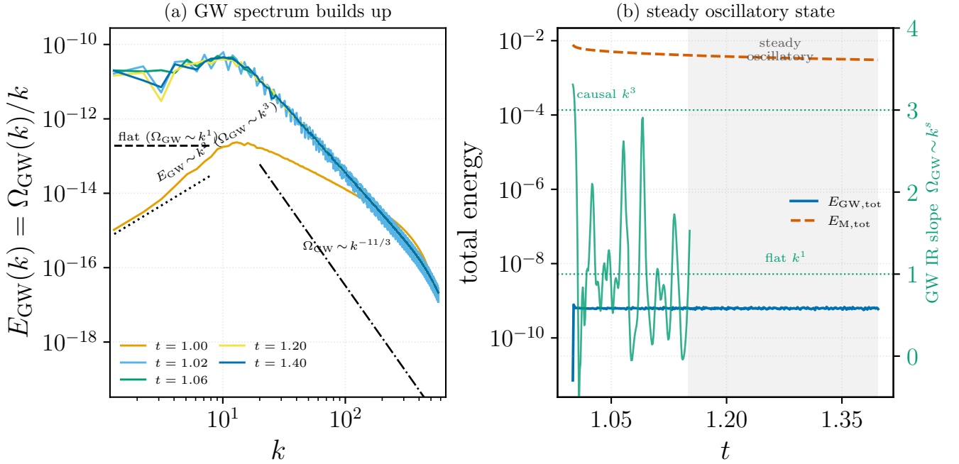
FIG. 11. Time-series reanalysis of the Roper Pol et al. [22] run ini2 (public Pencil Code spectra, Zenodo 10.5281/zenodo.3692072), the run of their Fig. 1. (a) The GW energy spectrum E_{\text{GW}} = \Omega_{\text{GW}}/k at successive times: at switch-on ( t \simeq 1.0 ) the infrared follows the causal E_{\text{GW}} \sim k^2 ( \Omega_{\text{GW}} \sim k^3 ) and within \Delta t \sim 0.02 saturates to the flat plateau ( \Omega_{\text{GW}} \sim k^1 ) of their Fig. 1. (b) Total energies versus time: the GW energy rises while the source acts, then fluctuates about a steady mean (grey band; the “steady oscillatory state”), while the magnetic energy keeps decaying; the right axis (green) shows the measured GW infrared slope crossing from the causal k^3 to the saturated k^1 . Generated by Notebooks/roperpol_timeseries.py , which auto-downloads the data.
