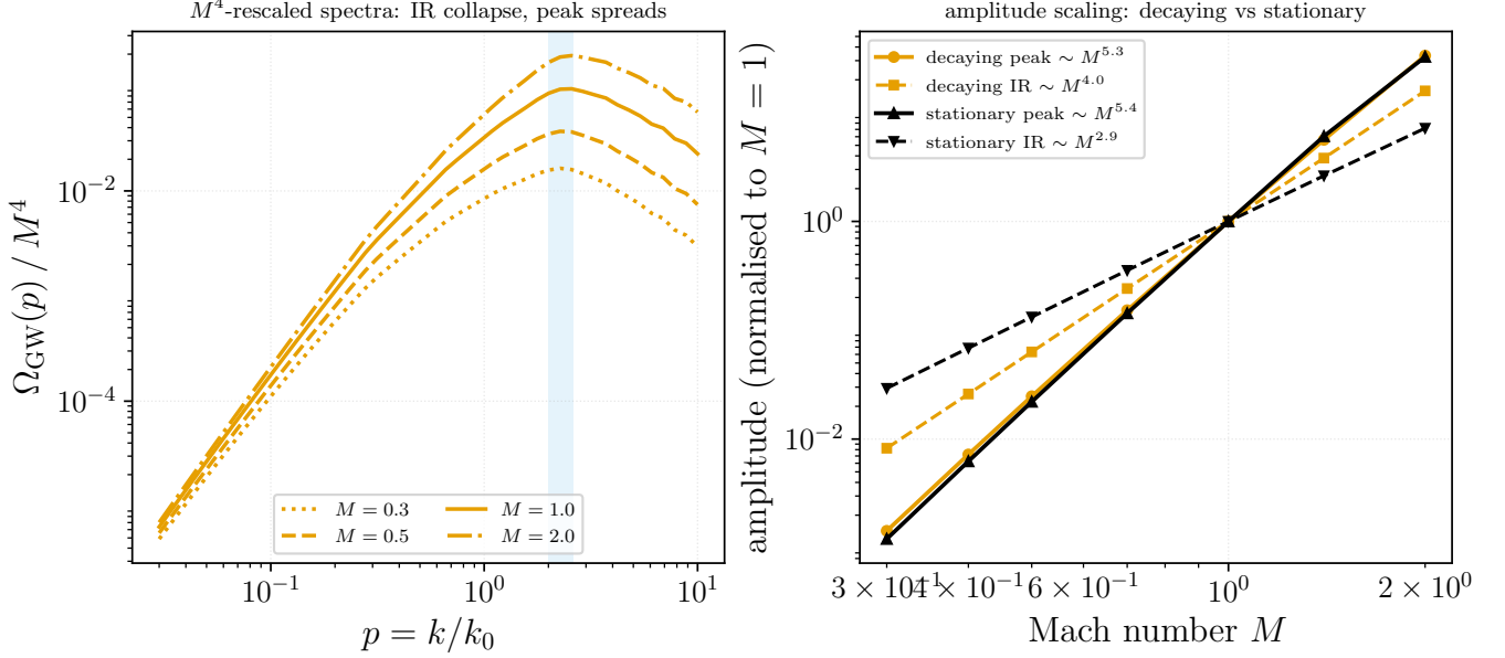
FIG. 7. Mach scaling of the full-spatial decaying GW amplitude, from the exact factorisation \Omega_{\text{GW}} = M^4 p^3 \Psi(p, p/M) [Eq. (34)]. (a) M^4 -rescaled spectra \Omega_{\text{GW}}(p)/M^4 for M = 0.3 – 2 ( R = 10^4 ): the curves collapse in the infrared—confirming the M^4 prefactor—and spread upward through the source-scale band (shaded), the peak amplitude growing faster than M^4 . (b) Amplitude versus M , normalised at M = 1 , with fitted power laws: the decaying infrared amplitude scales as M^{4.0} (one power above the stationary M^{2.9} ), while the source-pinned peak amplitude steepens to M^{5.3} . Generated by Notebooks/decaying_amplitude.py .
