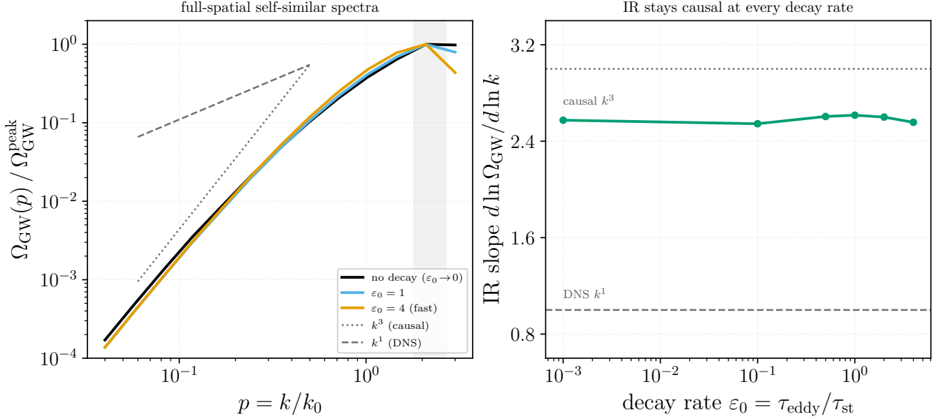
FIG. 10. The finite duration of a decaying source does not flatten the infrared. Left : GW spectra from the first-principles full-spatial self-similar kernel ( T_{\text{em}} = 40\tau_{e0} , M = 1 ) at three decay rates; the infrared slopes overlap on the causal k^3 guide (dotted) rather than the k^1 guide (dashed), and share the source-scale peak (shaded). Right : the infrared slope versus the decay rate \varepsilon_0 = \tau_{\text{eddy}}/\tau_{\text{st}} stays at the causal value ( \simeq 2.5 – 3 ) for every \varepsilon_0 , never approaching the simulated k^1 ; the physically realised self-similar decay sits at \varepsilon_0 \sim 1 . Generated by Notebooks/fullspatial_selfsimilar_exact.py .
