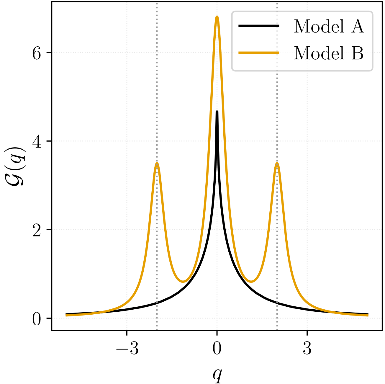
FIG. 1. Dimensionless temporal kernel \mathcal{G}(q) = \widehat{R^2}(q) for the two correlation models considered in Sec. IV. Model A uses the random-phase BK2016 form R_A(\sigma) = (1 + |\sigma|)^{-2/3} ; Model B is the coherent eddy R_B(\sigma) = \cos(\sigma) e^{-\alpha|\sigma|} with \alpha = 0.15 .
