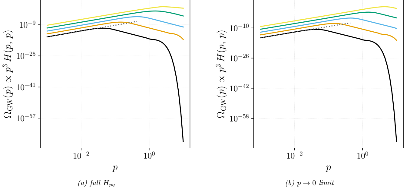
FIG. 6. Kraichnan decorrelation + Kolmogorov spectrum. Five curves per panel correspond to M = 0.03, 0.1, 0.3, 1.0, 3.0 at R = 10^4 . Panel (a) is the full numerical H_{pq} (Sec. II); panel (b) is the aeroacoustic p \rightarrow 0 limit (Kahniashvili et al. 2008). Both give the universal IR slope \Omega_{\text{GW}} \propto p^3 .
