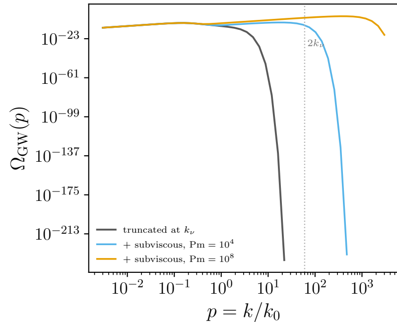
(a) the subviscous range radiates above 2k_\nu
