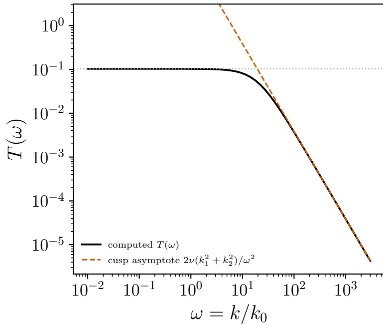
(b) the viscous factor is flat in the infrared
