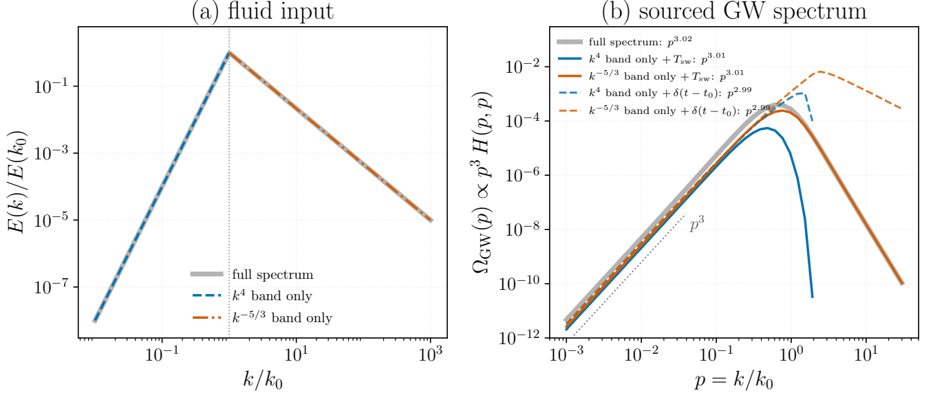
FIG. 18. Band-split test of the white-noise-floor hypothesis. (a) The three fluid inputs fed to the kernel: the full spectrum of Eq. (25) (grey), its Batchelor band E \propto k^4 alone (blue, dashed) and its Kolmogorov range E \propto k^{-5/3} alone (orange, dash-dotted), obtained by masking the shape factor S(k) = A(k)/A_{\text{Kol}}(k) on one side of k_0 (dotted vertical line). (b) The gravitational-wave spectra \Omega_{\text{GW}}(p) \propto p^3 H_{ijij}(p, p; M, R) they source on the sound-cone diagonal q = p , with the infrared log-log slopes fitted over 2 \times 10^{-3} \leq p \leq 2 \times 10^{-2} quoted in the legend; the dotted guide is p^3 . All are causal to better than 2% in the exponent, including the inertial-range-only run, whose input has no infrared power at all. The Batchelor-only spectrum ends at p = 2 , the kinematic limit of a convolution of two modes with k < k_0 . The two dashed curves repeat the single-band runs with the temporal factor removed entirely—evaluated at q = 0 rather than on the diagonal q = p , so that the Gaussian sweeping factor and its erfc in Eq. (23) are both unity and the source carries no decorrelation and no time dependence at all [the impulsive limit, Eq. (B105)]. The spatial integral is otherwise identical, so each solid/dashed pair isolates what the temporal model does and does not control. Parameters: M = 0.5 , R = (k_d/k_0)^{4/3} = 10^4 , R_{\text{IR}} = k_0/k_{\text{IR}} = 10^2 , Batchelor infrared slope s = 4 . Both panels are dimensionless and the vertical offset between them carries no physical meaning. Produced by Notebooks/band_split_gw.py .
