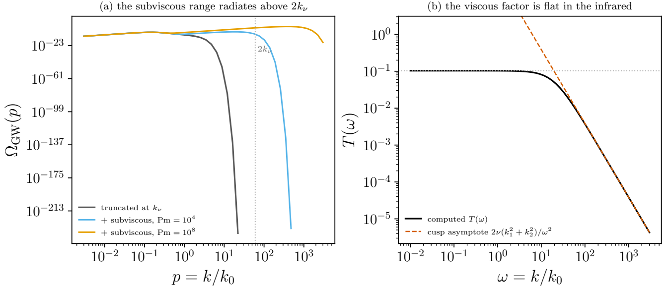
FIG. 20. (a) Adding a \text{Pm} \gg 1 subviscous magnetic range to a fixed large-scale field changes \Omega_{\text{GW}} only above p \simeq 2k_\nu/k_0 ; the infrared is untouched. (b) The two-leg viscous temporal factor, computed rather than extrapolated: flat below 1/\tau_c , so it adds no power of k where the observations are.
