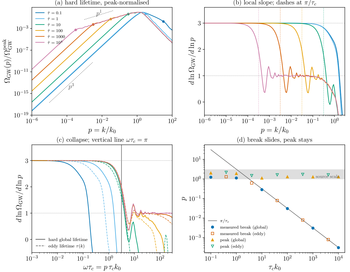
FIG. 14. Local logarithmic slope of \Omega_{\text{GW}} against p = k/k_0 for the triangular (finite-lifetime) correlator, at several \hat{\tau} = \tau_c k_0 . The slope sits at 3 in the infrared and falls to 1 above the break Eq. (45); the residual oscillation about the linear band is the \sin^2 ringing of the finite window, not noise. The linear band is resolved only for \hat{\tau} \gtrsim 10^3 .
