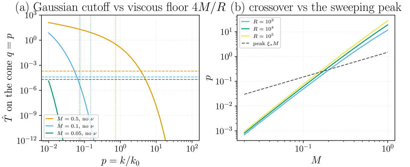
FIG. 21. The viscous cusp. (a) The two-leg sweeping factor on the cone q = p (solid) against the viscous floor 4M/R of Eq. (56) (dashed) at R = 10^4 ; dotted verticals mark the sweeping peak \xi_* M . The Gaussian is super-exponential in p^{2/3}/M^2 , so the constant floor overtakes it, and the more subsonic the flow the earlier. (b) The crossover against M for three Reynolds numbers, with the peak \xi_* M dashed: the floor emerges above the peak for M \gtrsim 0.3 and below it for M \lesssim 0.1 . Temporal factor only — the full two-wavevector kernel is not evaluated here. Generated by Notebooks/viscous_cusp_floor.py .
