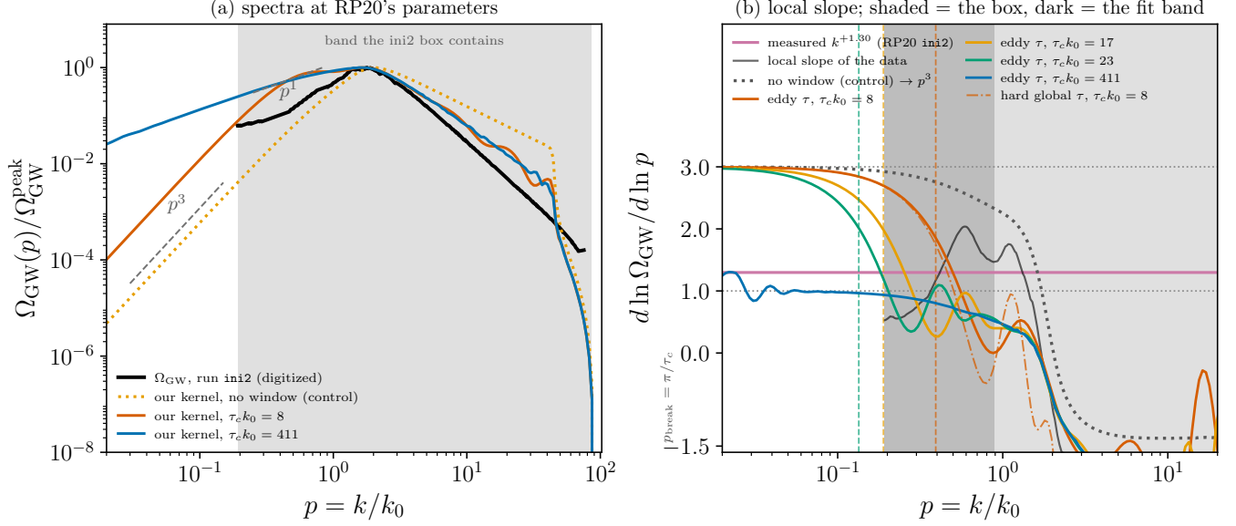
FIG. 15. The kernel of this paper at Ref. [28]’s own parameters. (a) The digitised ini2 spectrum against our kernel at \hat{\tau} = 8 and 411 and against the no-window control, with the band the box contains shaded and p^1 , p^3 guides. (b) Local logarithmic slope: the four lifetime closures, the control tending to +3, the smoothed local slope of the data, and the measured band average +1.30; vertical dashes mark p_{\text{break}} = \pi/\tau_c for each closure, and the dark shading is the fit band. The control already fails to reach +3 inside the box, which is the point of panel (b).
