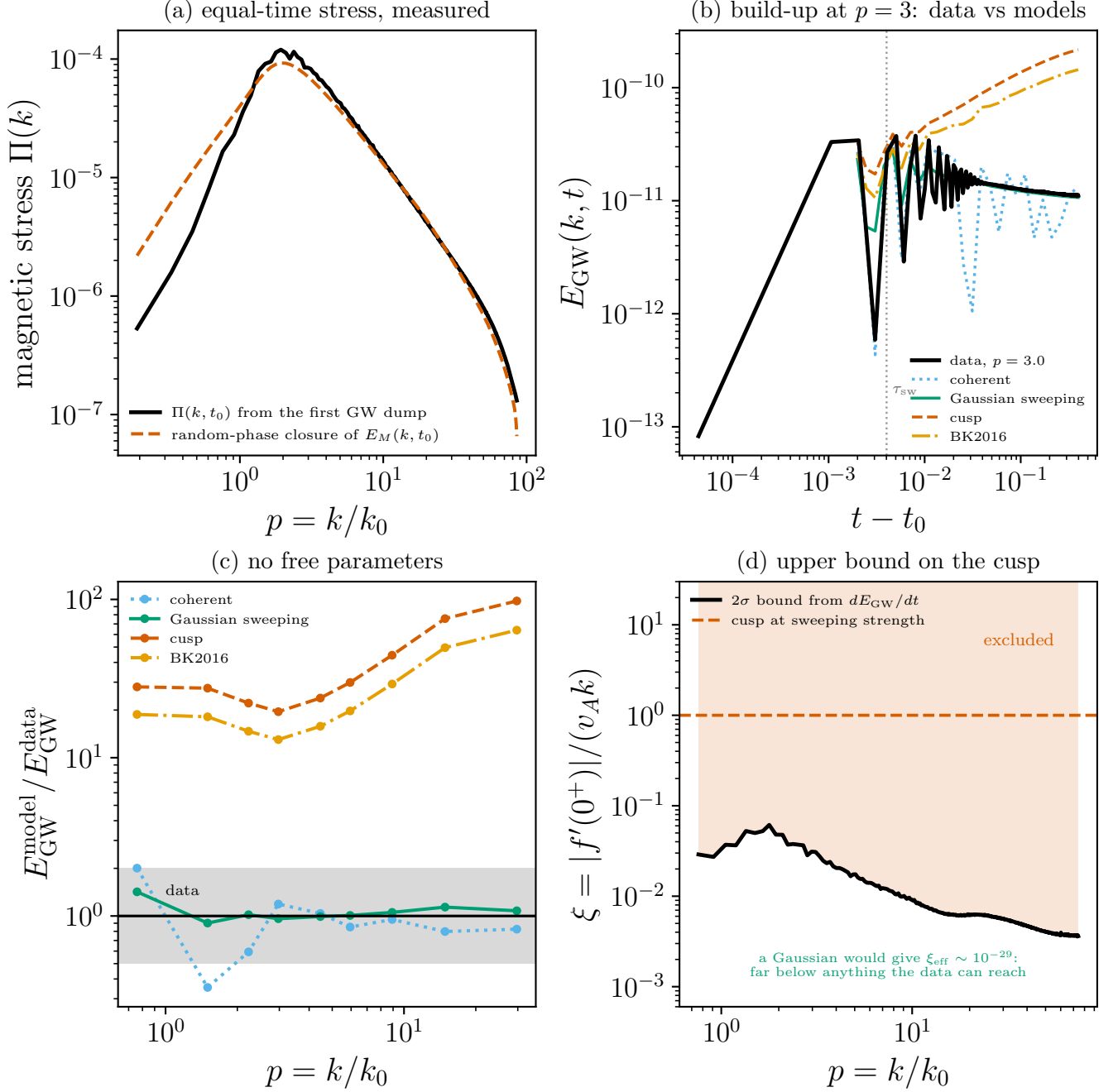
FIG. 11. Parameter-free forward models of run ini2 's GW spectrum from its own measured magnetic stress. Cuspless correlators reproduce the data; cusped ones overpredict by one to two orders of magnitude.
