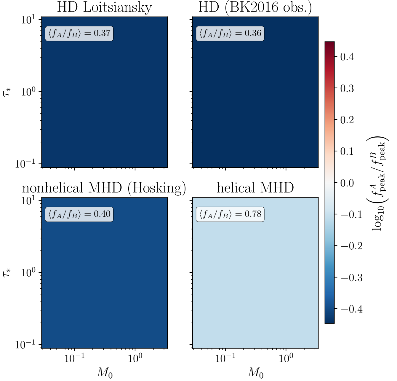
FIG. 23. Model A/B ratio of the peak GW frequency, \log_{10}(f_{\text{peak}}^A / f_{\text{peak}}^B) , on the (\tau_*, M_0) plane for the four BK2016 self-similar decay classes (HD Loitsiansky q = 2/7 , \beta = 4 ; the HD class realised in the simulations of Ref. [39] q = 1/3 , \beta = 3 ; nonhelical MHD q = 4/9 , \beta = 3/2 , the Hosking-integral class; helical MHD q = 2/3 , \beta = 0 ). HD Saffman q = 1/3 , \beta = 3 ; nonhelical MHD q = 1/2 , \beta = 1 ; [the caption still documented the superseded q = 1/2 , \beta = 1 magnetic class that the code no longer plots, and named the \beta = 3 panel “Saffman”, which it is not ( \beta = 2 , q = 2/5 )] Each panel is flat: the ratio is independent of (\tau_*, M_0) , fixed only by the kernel shapes, with the per-class value \langle f_A/f_B \rangle annotated. Model A (random-phase) peaks below Model B (coherent eddy) everywhere. The offsets group as 0.37, 0.36, 0.40, 0.78: three classes together and helical MHD apart, not HD against MHD. the HD-classes show the larger offset [the old clause restated the HD-versus-MHD split that the text two paragraphs above now explicitly retracts]
