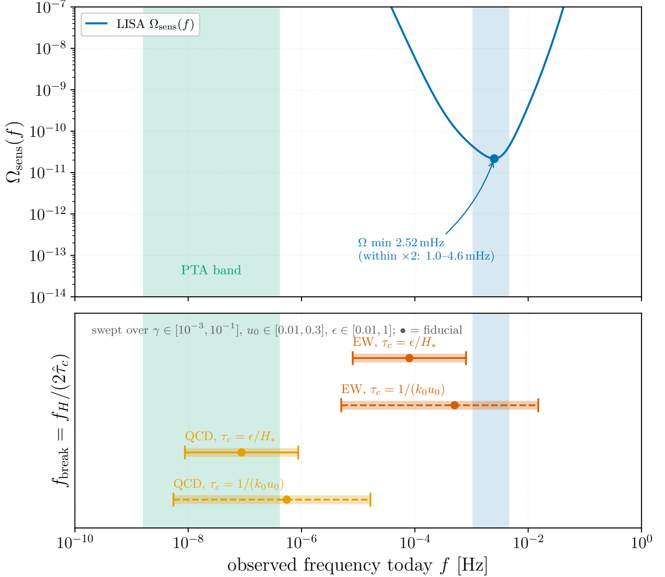
FIG. 17. Where the break falls relative to the observing bands. Top : the LISA energy-density sensitivity \Omega_{\text{sens}}(f) from the SciRD analytic noise model, with its minimum at 2.52 mHz and the factor-of-two window shaded, and the pulsar-timing band. Bottom : f_{\text{break}} swept over the parameter ranges of Table VI for the two epochs and the two lifetime closures. The bands are two to three decades wide, which is the point: the break’s position relative to each instrument is robust where its value is not. Generated by Notebooks/k_break_frequency.py .
