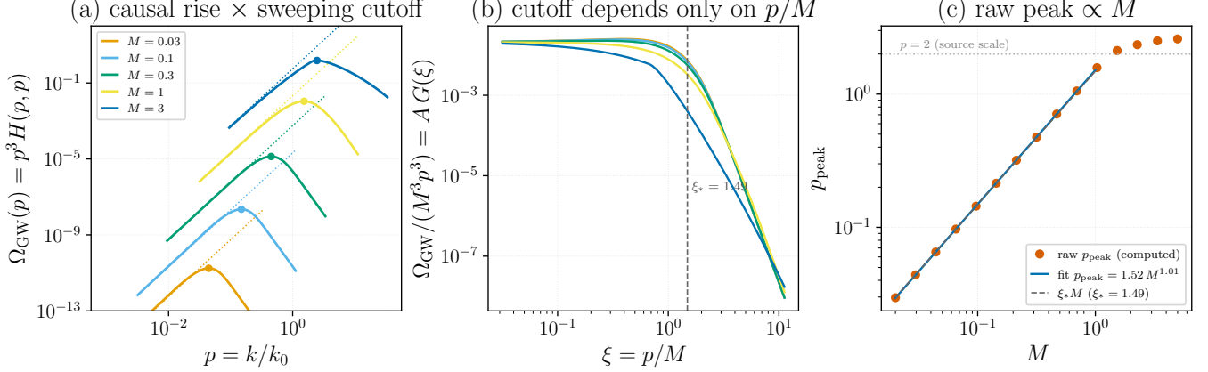
FIG. 3. Why the stationary GW spectrum peaks at p \simeq 1.49 M rather than at the source scale p \sim 2 , computed from \Omega_{\text{GW}}(p) = p^3 H_{ijij}(p, p; M, R) [Eq. (23), R = 10^4 ]. (a) Each spectrum (solid) follows its causal infrared asymptote A M^3 p^3 (dotted) and rolls over at the peak (dot) where the sweeping cutoff switches on. (b) Collapse: \Omega_{\text{GW}}/(M^3 p^3) = \tilde{H}_{ijij}(p, p; M)/M^3 versus \xi = p/M falls on the single compensated kernel \tilde{H}_{ijij}(\xi) for every M , proving the cutoff depends only on p/M [Eq. (28)]; the universal peak position is \xi_* = 1.488 . (c) Peak location read directly from each computed spectrum (points) versus M : a power law p_{\text{peak}} = 1.515 M^{1.007} (line) [Eq. (31)], coincident with \xi_* M (dashed), that bends below it toward the p = 2 source scale (dotted) only as M \rightarrow 1 (the luminal limit; M > 1 is superluminal). Generated by Notebooks/stationary_peak_analysis.py .
