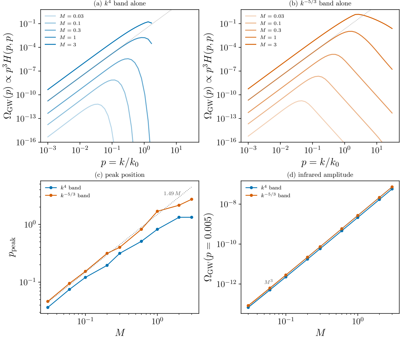
FIG. 19. Mach dependence of the band-split spectra, at R = 10^4 , R_{\text{IR}} = 10^2 , Kraichnan sweeping on the diagonal q = p . (a), (b) \Omega_{\text{GW}}(p) from the Batchelor k^4 band alone and from the Kolmogorov k^{-5/3} band alone, at M = 0.03, 0.1, 0.3, 1, 3 (increasing shade); dotted line p^3 . The infrared exponent is M -independent for both bands; the amplitude and the peak are not. (c) Peak position against M , with the 1.49 M sweeping law of Eq. (31) dotted. The inertial band reproduces it; the Batchelor band tracks a slightly lower 1.1 M and saturates above M \simeq 1 , where the sweeping scale meets the kinematic ceiling p \leq 2 that bounds a convolution of two modes with k < k_0 . (d) Infrared amplitude at p = 5 \times 10^{-3} against M , with the M^3 prefactor dotted; both bands follow it to 16.6% and 14.0% over two decades of M . Produced by Notebooks/band_split_mach.py .
