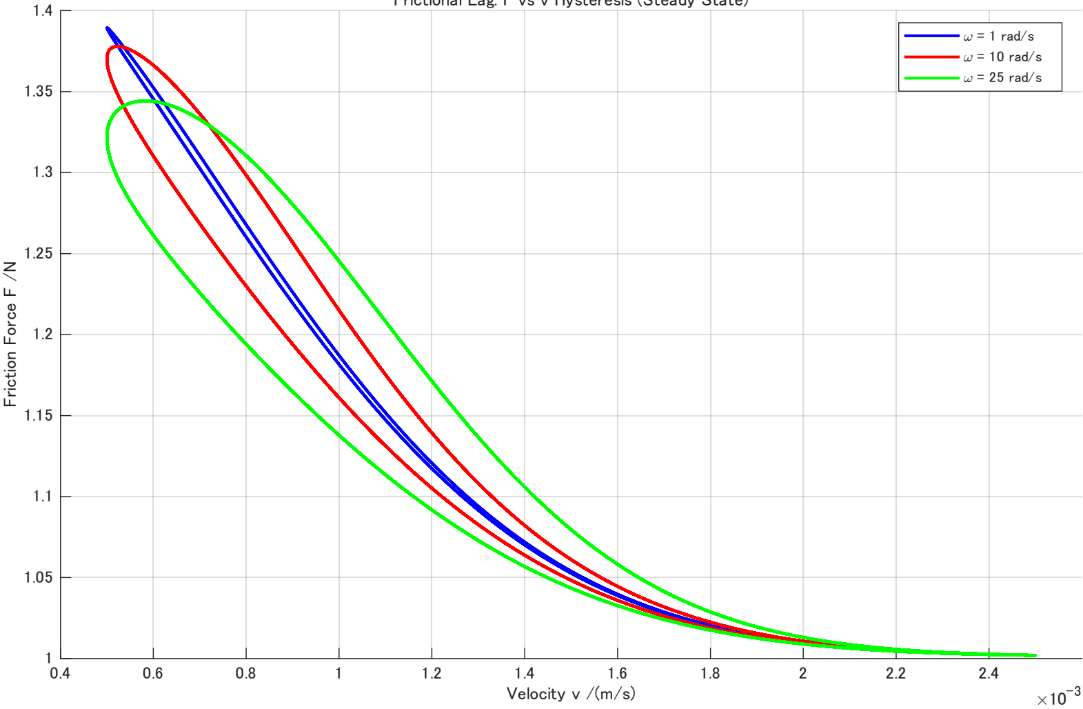
Frictional Lag: F vs v Hysteresis (Steady State)
