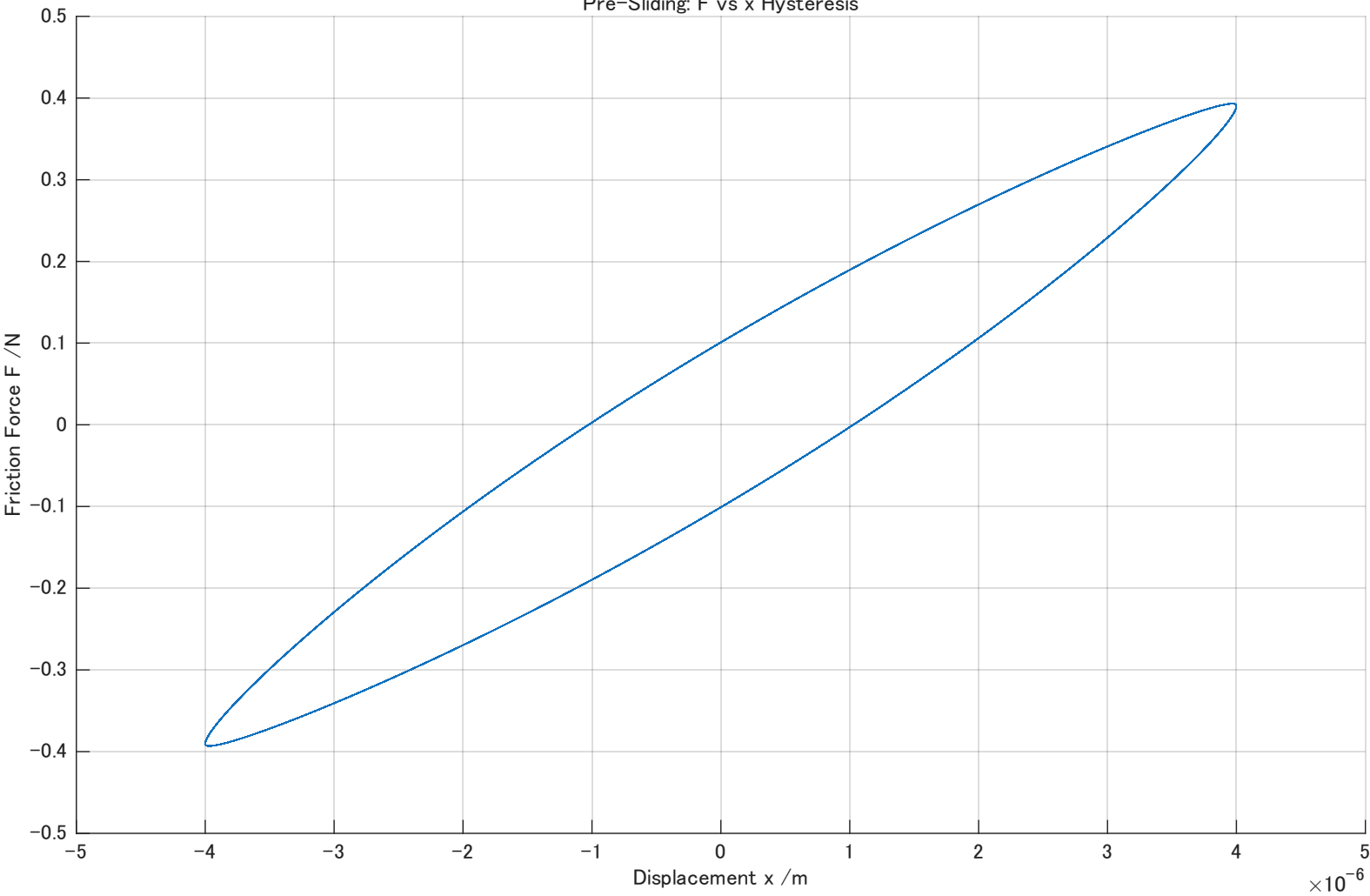
Pre-Sliding: F vs x Hysteresis
