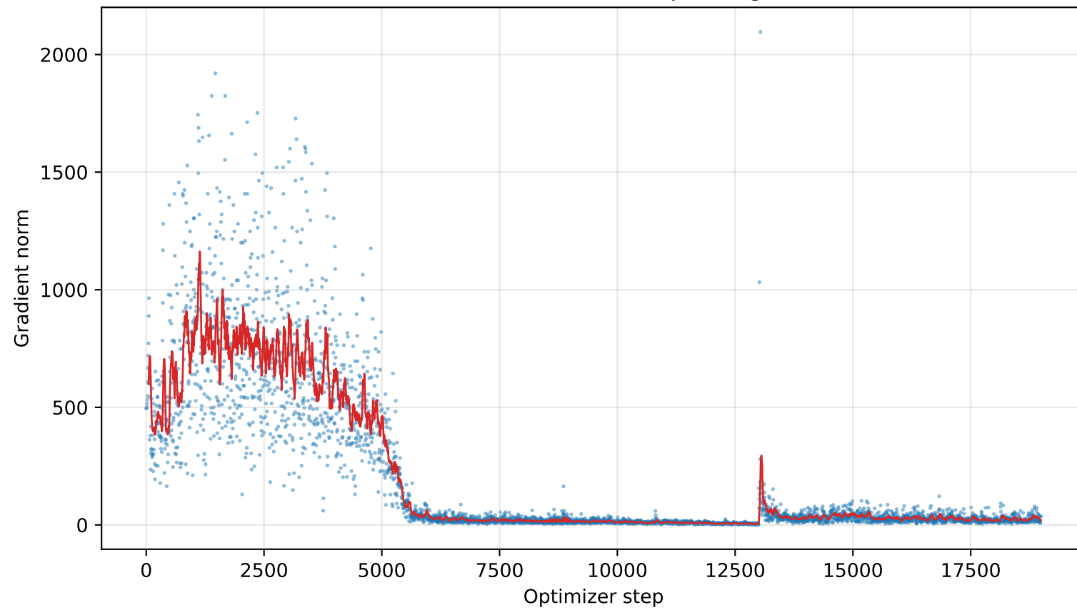
Gradient norm (50-step rolling)
