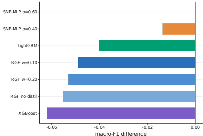
d Gap to best macro-F1
