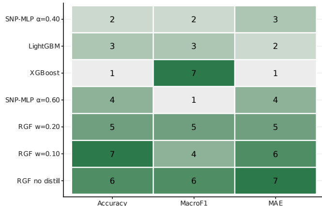
c Rank depends on metric
