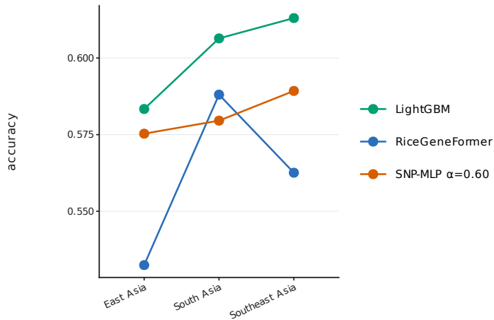
c Accuracy under region shift
