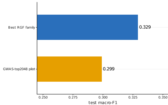
d GWAS-top2048 replacement did not help
