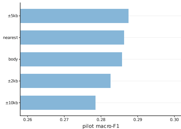
c Mapping window: no stable winner
