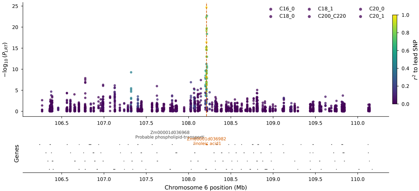
R01_Zm00001d036982: Zm00001d036982 (6:106,212,452-110,212,452)
