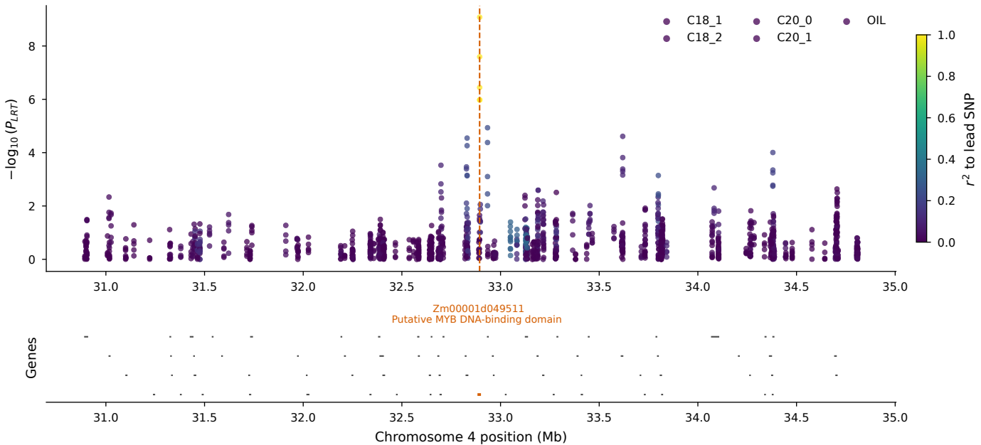
R02_Zm00001d049511: Zm00001d049511 (4:30,894,031-34,894,031)
