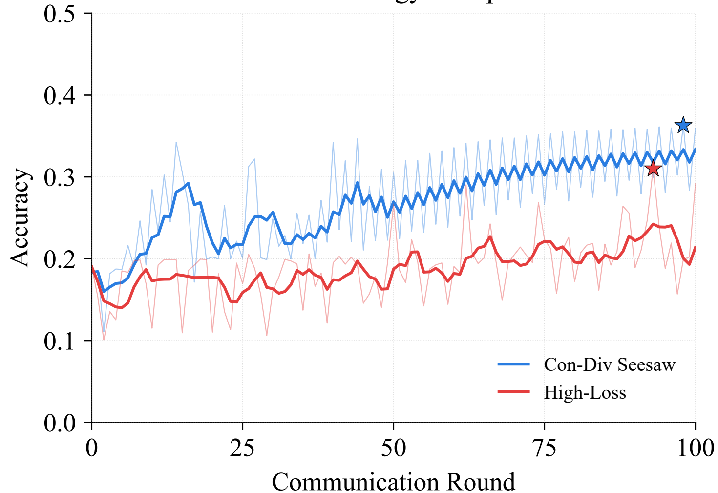
FMNIST Strategy Comparison
